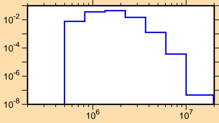
\sigma vs. E for ^{139}\text{Ce}(n,n_3)
