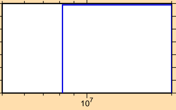
\sigma vs. E for ^{139}\text{Ce}(n,2np)
