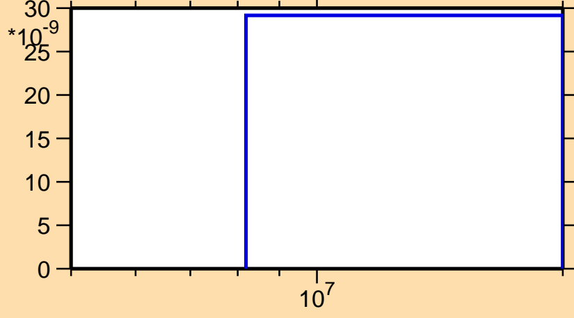
\sigma vs. E for ^{139}\text{Ce}(n,\text{nd})
