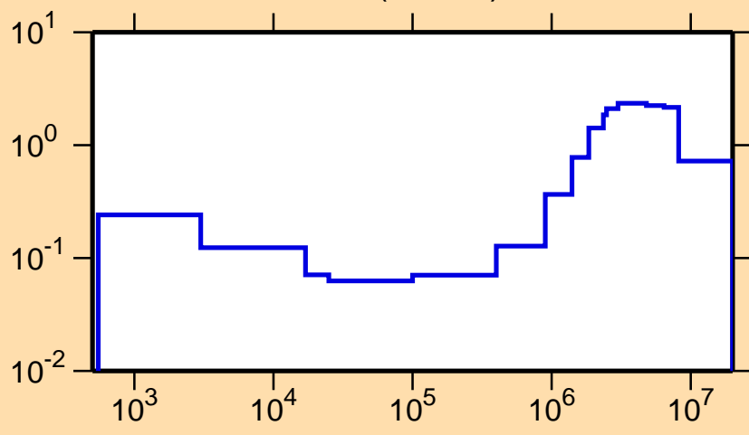
\sigma vs. E for ^{139}\text{Ce}(n,\text{inel.})
