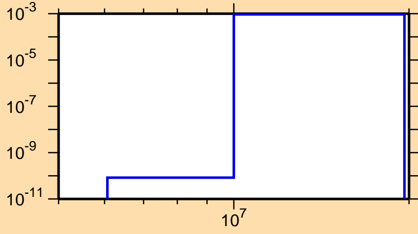
\sigma vs. E for ^{140}\text{Ce}(n,d)
