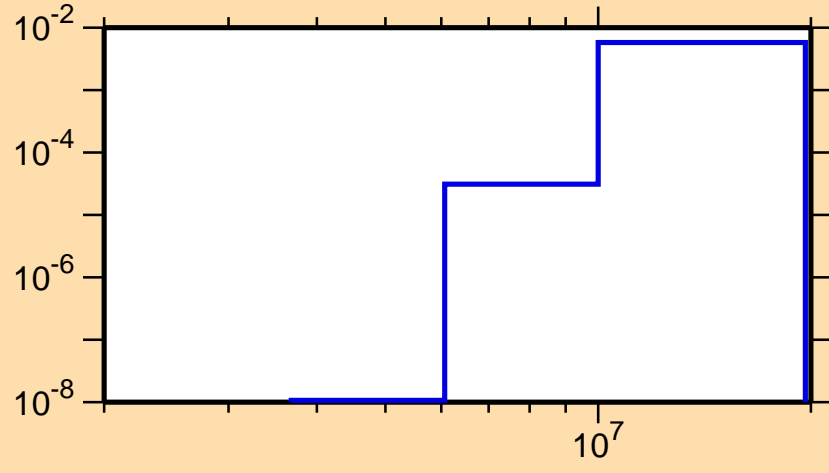
\sigma vs. E for ^{140}\text{Ce}(n,p)
