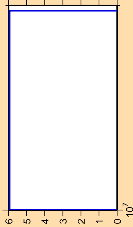
\Delta\sigma/\sigma vs. E for ^{140}\text{Ce}(n,2np)
