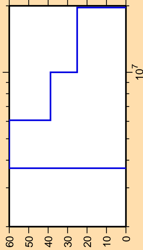
\Delta\sigma/\sigma vs. E for ^{140}\text{Ce}(n,p)
