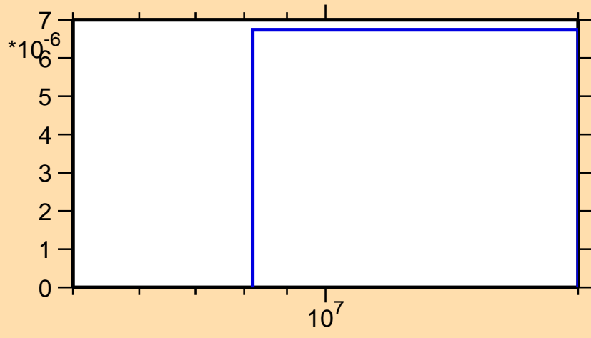
\sigma vs. E for ^{140}\text{Ce}(n,t)
