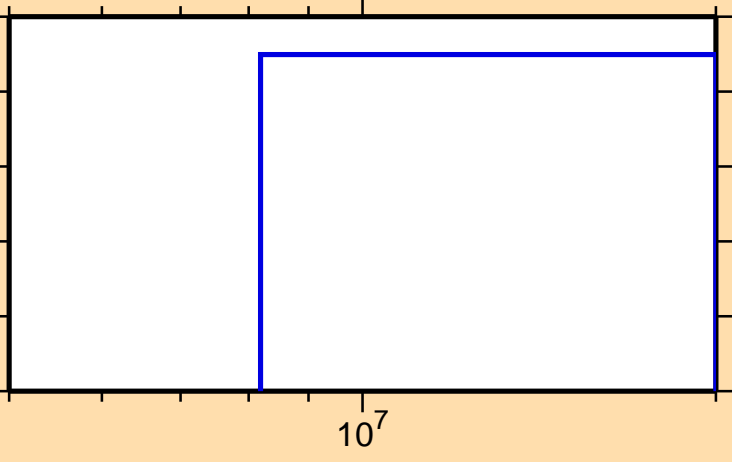
\sigma vs. E for ^{140}\text{Ce}(n,np)
