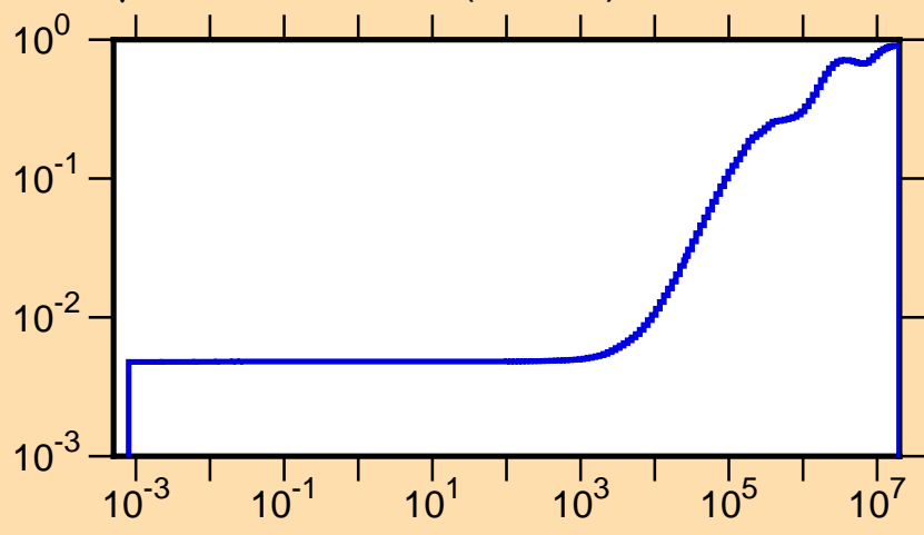
\mu vs. E for ^{141}\text{Ce}(\text{mt251})
