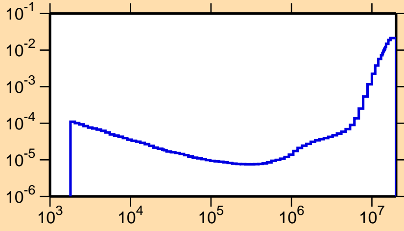
\sigma vs. E for ^{141}\text{Ce}(n,\alpha)
