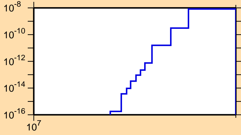
\sigma vs. E for ^{141}\text{Ce}(n,\text{He3})
