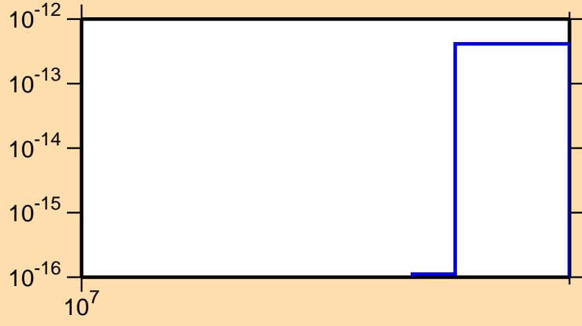
\sigma vs. E for ^{141}\text{Ce}(n,\text{pt})
