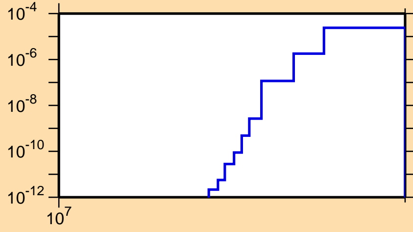
\sigma vs. E for ^{141}\text{Ce}(n,\text{nd})
