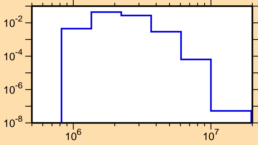
\sigma vs. E for ^{141}\text{Ce}(n,n_2)
