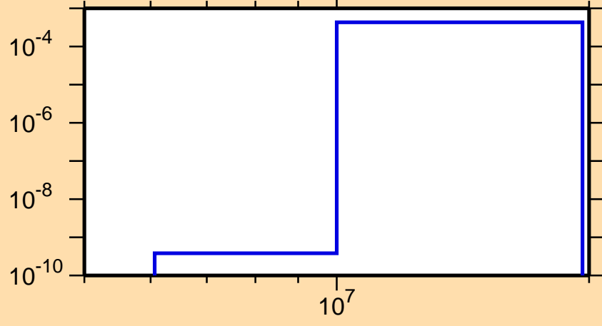
\sigma vs. E for ^{141}\text{Ce}(n,t)
