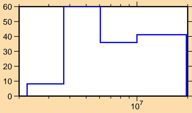
\Delta\sigma/\sigma vs. E for ^{141}\text{Ce}(n,p)
