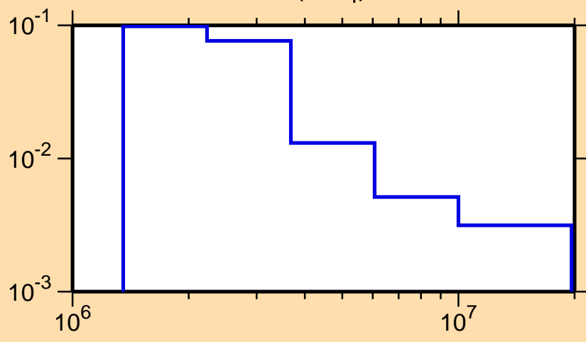
\sigma vs. E for ^{141}\text{Ce}(n,n_4)
