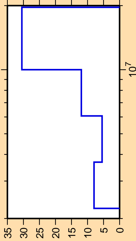
\Delta\sigma/\sigma vs. E for ^{141}\text{Ce}(n,n\text{cont.})
