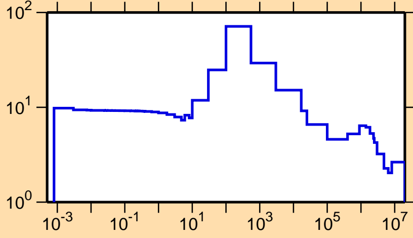
\sigma vs. E for ^{141}\text{Ce}(n,\text{el.})
