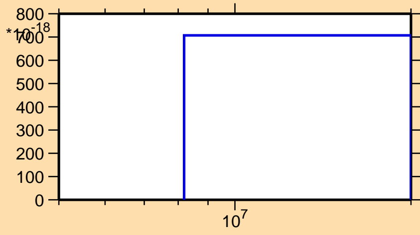
\sigma vs. E for ^{141}\text{Ce} (mt 34)
