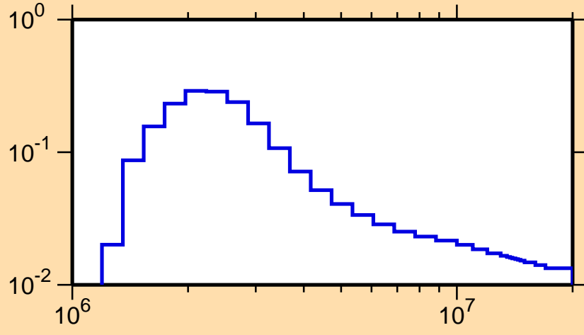
\sigma vs. E for ^{142}\text{Ce}(n,n_2)
