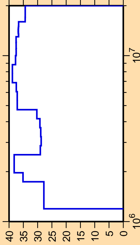
\Delta\sigma/\sigma vs. E for ^{142}\text{Ce}(n,n_2)
