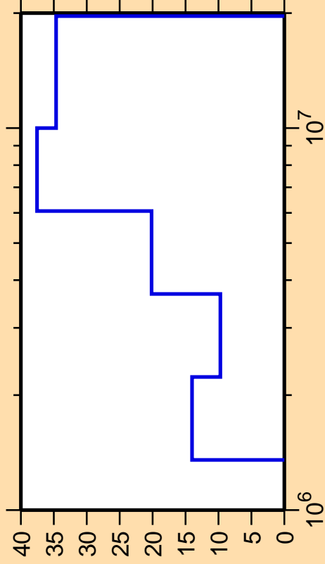
\Delta\sigma/\sigma vs. E for ^{142}\text{Ce}(n,n_4)
