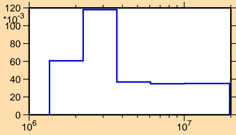
\sigma vs. E for ^{142}\text{Ce}(n,n_4)
