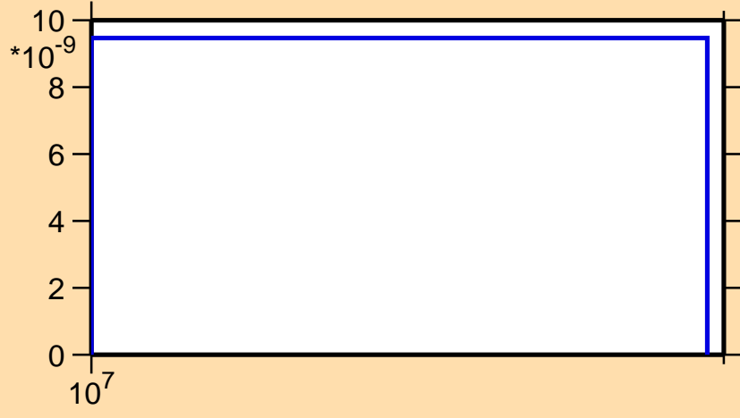
\sigma vs. E for ^{142}\text{Ce}(n,\text{nd})
