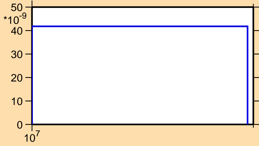
\sigma vs. E for ^{142}\text{Ce}(n,nt)
