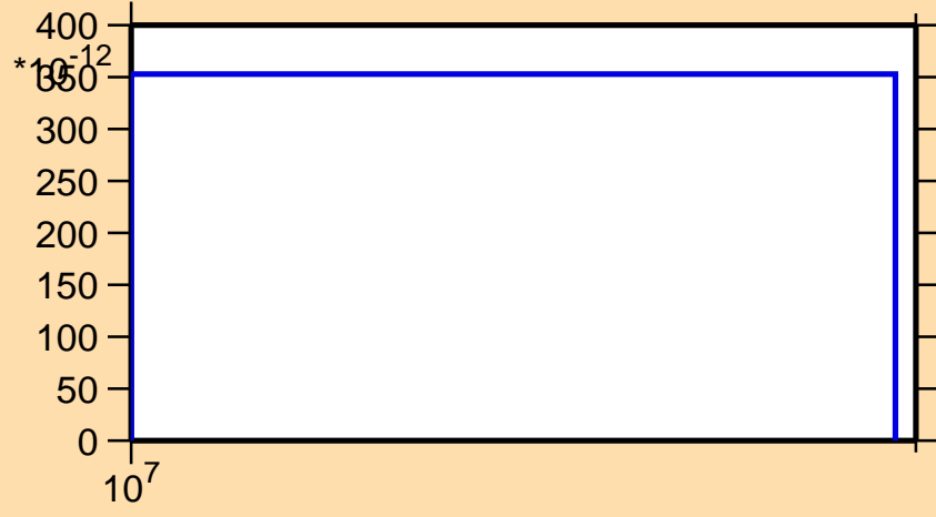
\sigma vs. E for ^{142}\text{Ce}(n,2np)
