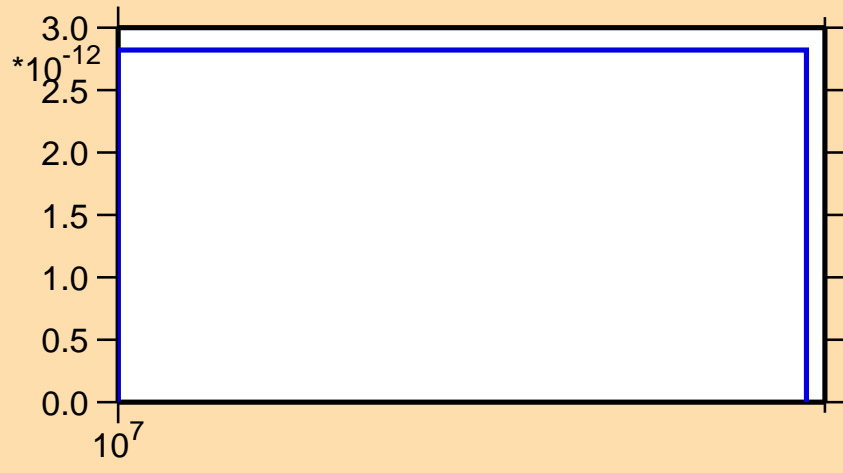
\sigma vs. E for ^{142}\text{Ce} (mt 45)
