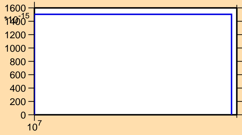
\sigma vs. E for ^{142}\text{Ce}(n,\text{He}3)
