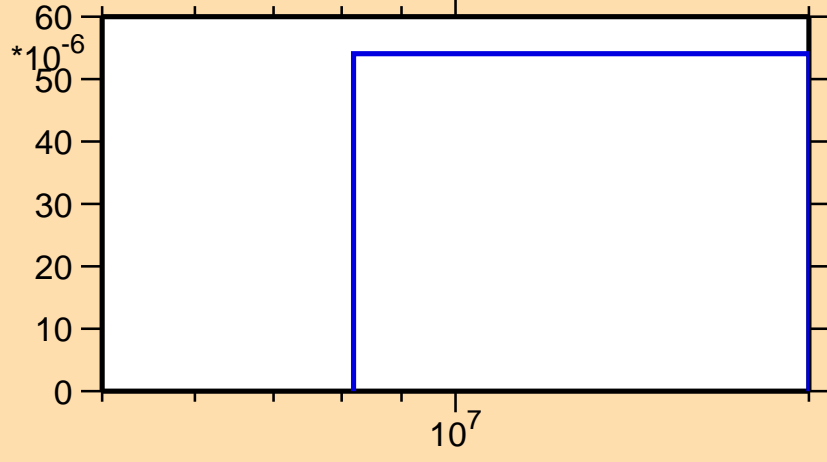
\sigma vs. E for ^{142}\text{Ce}(n,t)
