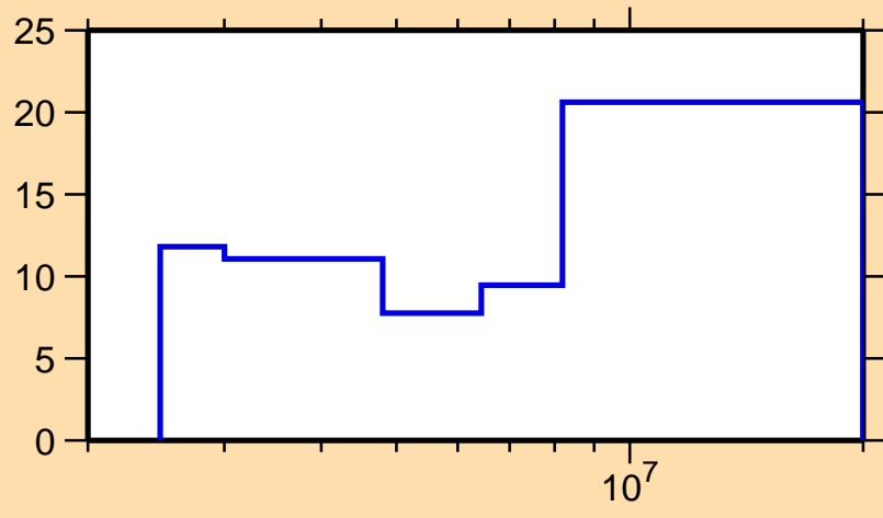
\Delta\sigma/\sigma vs. E for ^{142}\text{Ce}(n,n\text{cont.})
