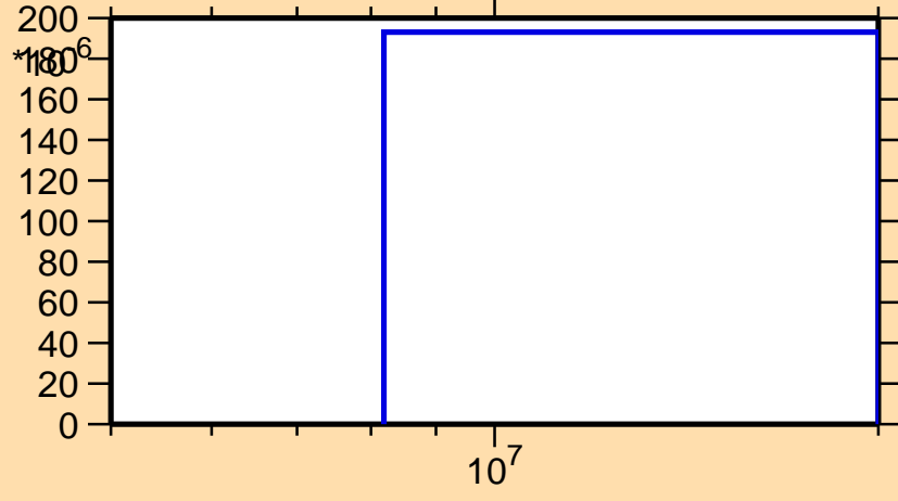
\sigma vs. E for ^{142}\text{Ce}(n,np)
