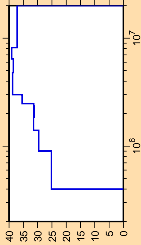
\Delta\sigma/\sigma vs. E for ^{142}\text{Ce}(n,n_1)
