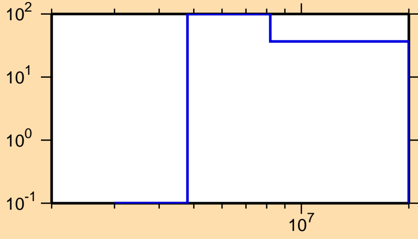
\Delta\sigma/\sigma vs. E for ^{142}\text{Ce}(n,p)
