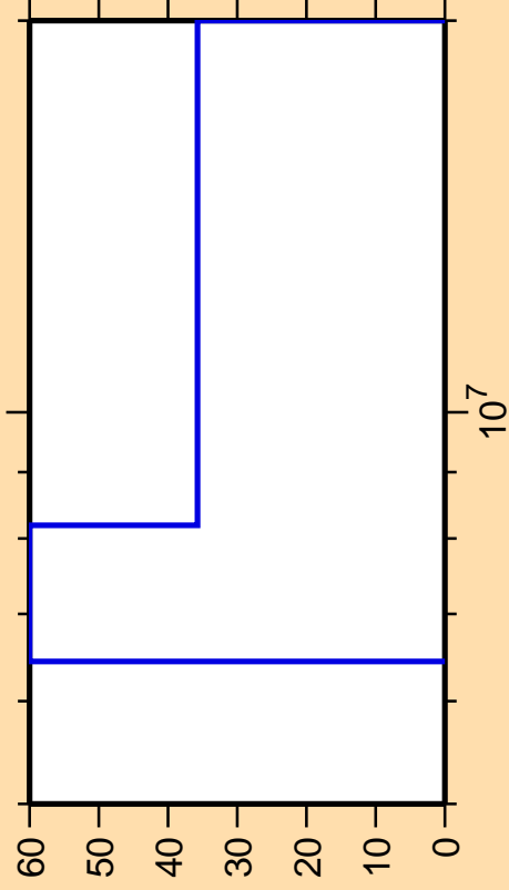
\Delta\sigma/\sigma vs. E for ^{142}\text{Ce}(n,\alpha)
