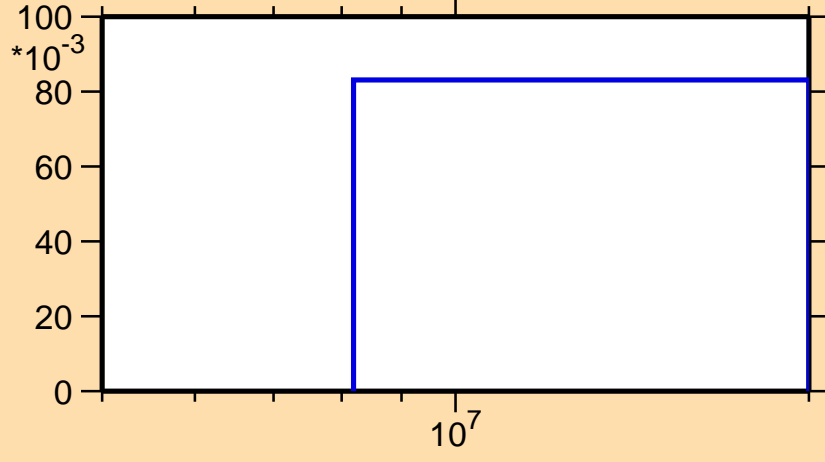
\sigma vs. E for ^{142}\text{Ce}(n,3n)
