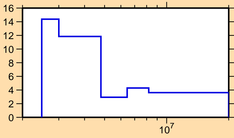
\Delta\sigma/\sigma vs. E for ^{142}\text{Ce}(n,\text{tot.})
