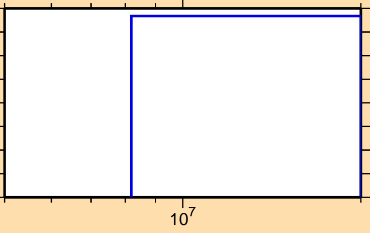
\sigma vs. E for ^{142}\text{Ce}(n,nt)
