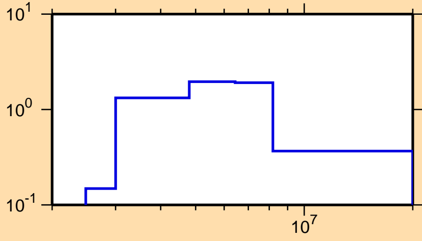
\sigma vs. E for ^{142}\text{Ce}(n,n\text{cont.})
