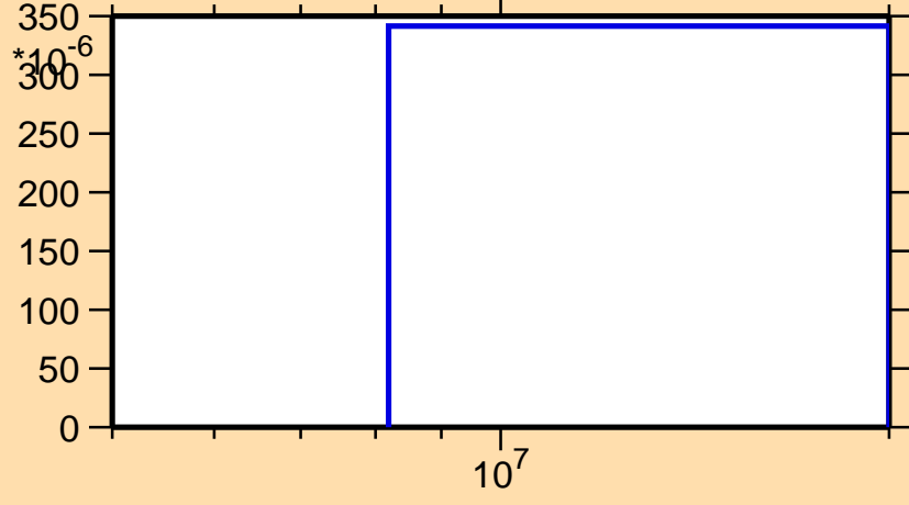
\sigma vs. E for ^{142}\text{Ce}(n,d)
