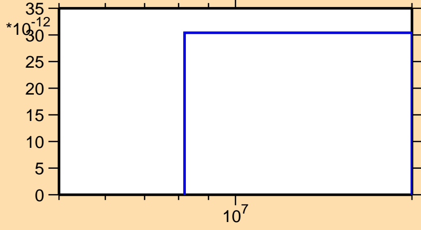
\sigma vs. E for ^{142}\text{Ce}(\text{mt117})
