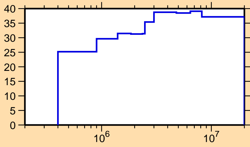
\Delta\sigma/\sigma vs. E for ^{142}\text{Ce}(n,n_1)
