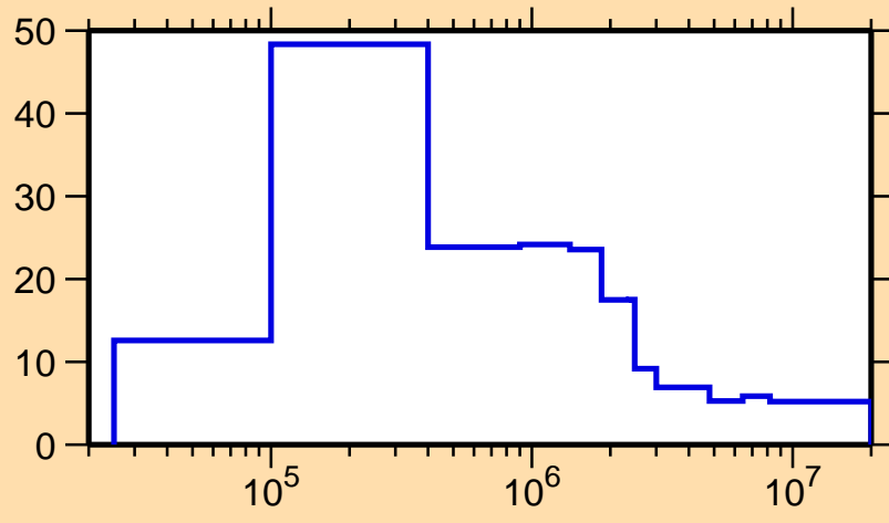
\Delta\sigma/\sigma vs. E for ^{142}\text{Ce}(n,\text{nonel.})
