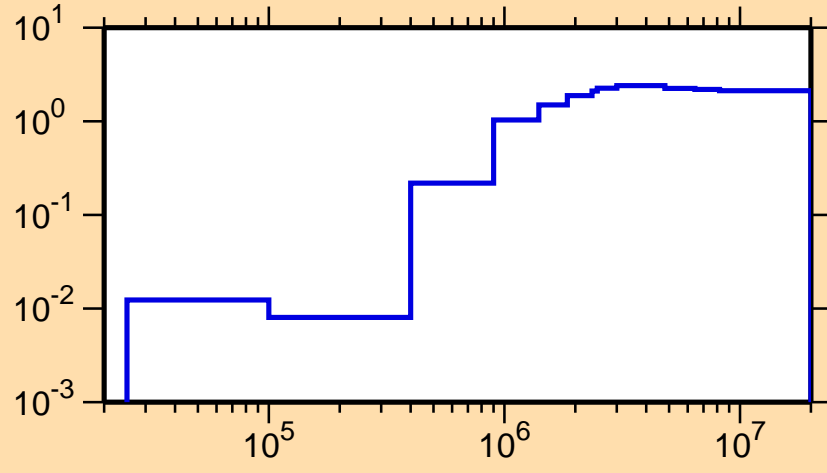
\sigma vs. E for ^{142}\text{Ce}(n,\text{nonel.})
