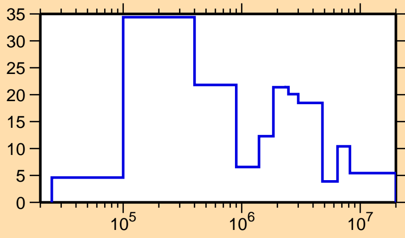
\Delta\sigma/\sigma vs. E for ^{142}\text{Ce}(n,\text{el.})
