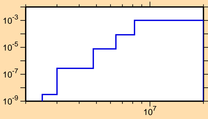
\sigma vs. E for ^{142}\text{Ce}(n,n\alpha)
