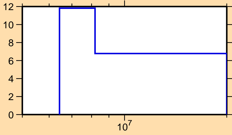
\Delta\sigma/\sigma vs. E for ^{142}\text{Ce}(n,2n)
