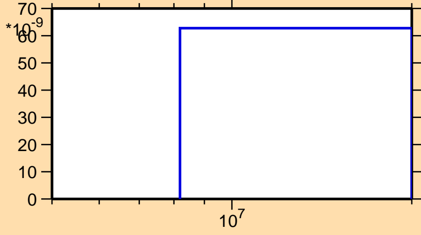
\sigma vs. E for ^{142}\text{Ce}(n,2n\alpha)
