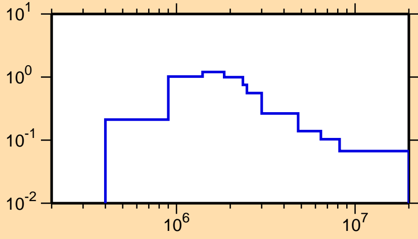
\sigma vs. E for ^{142}\text{Ce}(n,n_1)
