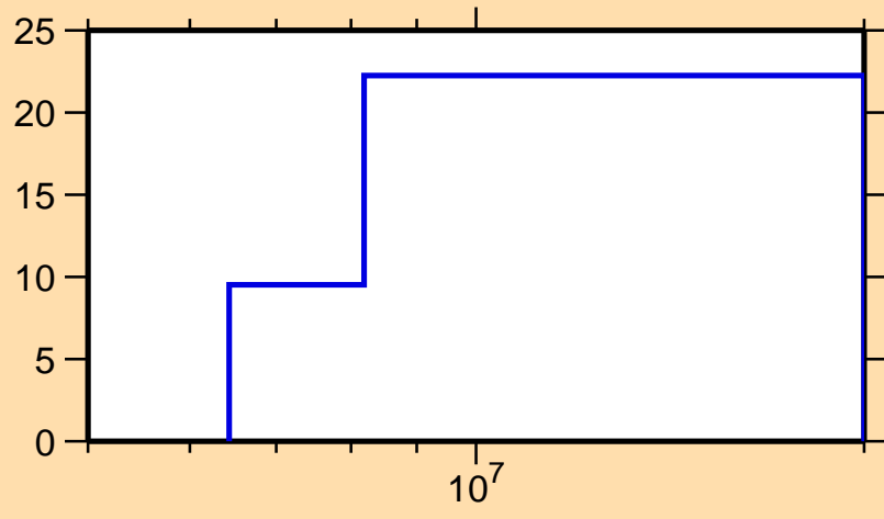
\Delta\sigma/\sigma vs. E for ^{142}\text{Ce}(n,\text{inel.})
