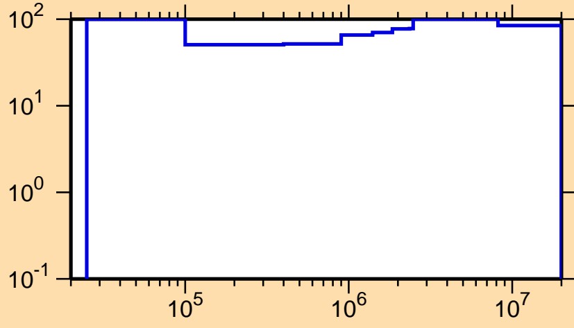
\Delta\sigma/\sigma vs. E for ^{142}\text{Ce}(n,\gamma)
