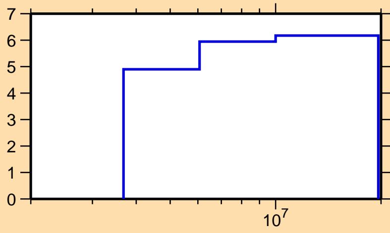
\Delta\sigma/\sigma vs. E for ^{143}\text{Ce}(n,\text{nonel.})
