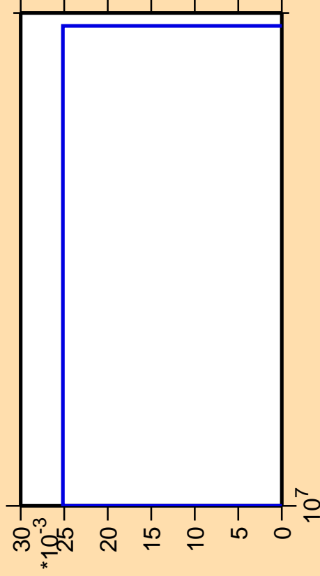
\Delta\sigma/\sigma vs. E for ^{143}\text{Ce}(\text{mt117})
