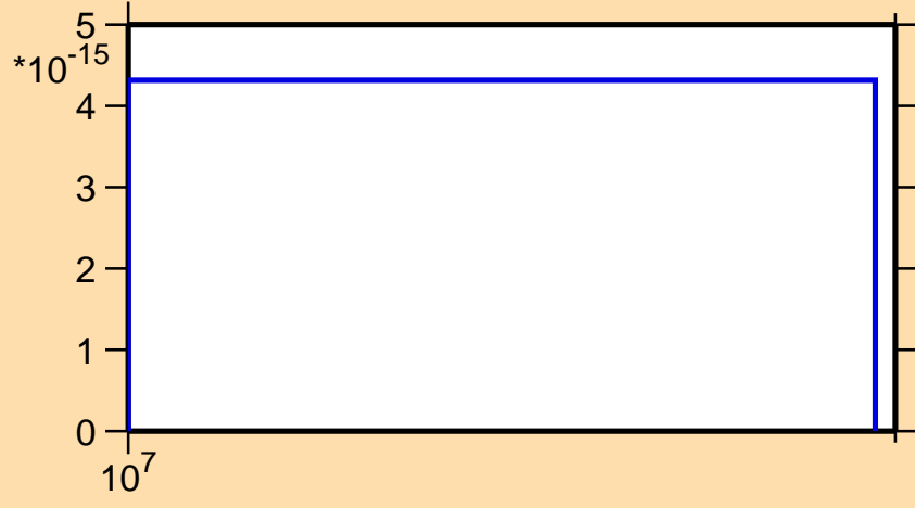
\sigma vs. E for ^{143}\text{Ce}(\text{mt117})
