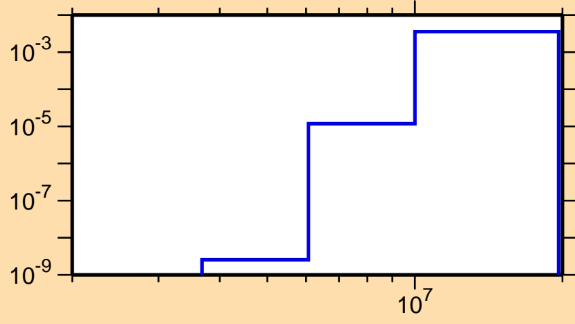
\sigma vs. E for ^{143}\text{Ce}(n,p)
