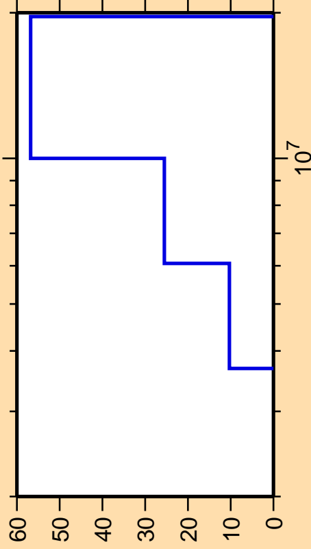
\Delta\sigma/\sigma vs. E for ^{143}\text{Ce}(n,n\text{cont.})
