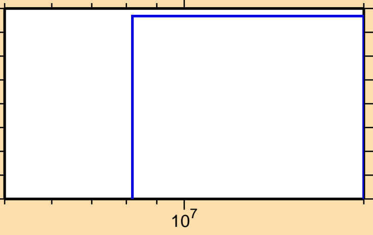
\sigma vs. E for ^{143}\text{Ce}(\text{mt117})
