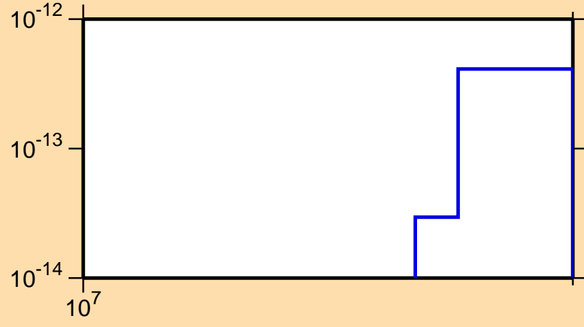
\sigma vs. E for ^{144}\text{Ce}(n,p\alpha)
