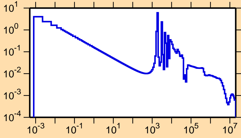
\sigma vs. E for ^{144}\text{Ce}(n,\gamma)
