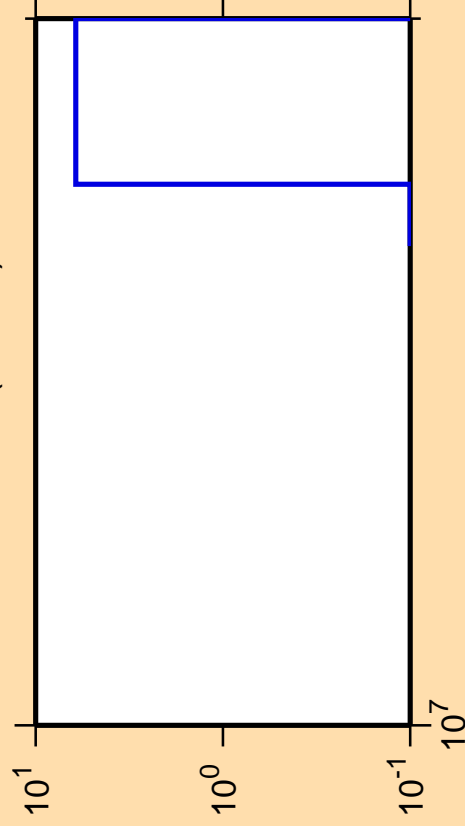
\Delta\sigma/\sigma vs. E for ^{144}\text{Ce}(n,\text{He}3)
