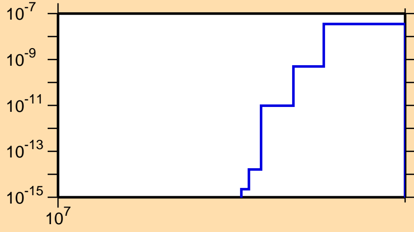
\sigma vs. E for ^{144}\text{Ce}(n,3n\alpha)
