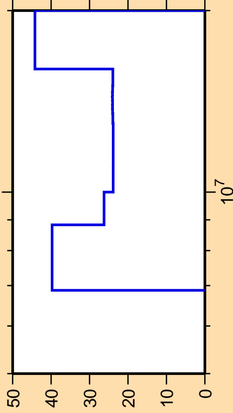
\Delta\sigma/\sigma vs. E for ^{144}\text{Ce}(n,2n)
