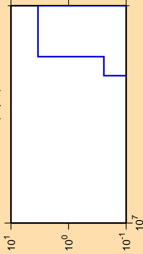
\Delta\sigma/\sigma vs. E for ^{144}\text{Ce}(n,p\alpha)
