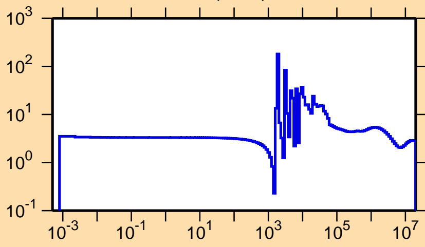
\sigma vs. E for ^{144}\text{Ce}(n,\text{el.})
