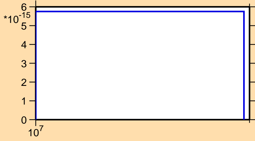
\sigma vs. E for ^{144}\text{Ce}(n,p\alpha)
