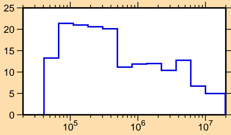
\Delta\sigma/\sigma vs. E for ^{144}\text{Ce}(n,\text{tot.})
