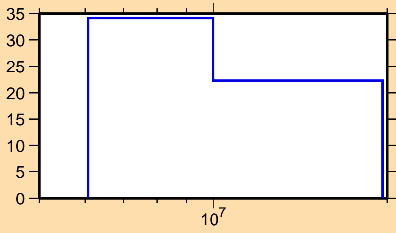
\Delta\sigma/\sigma vs. E for ^{144}\text{Ce}(n,2n)
