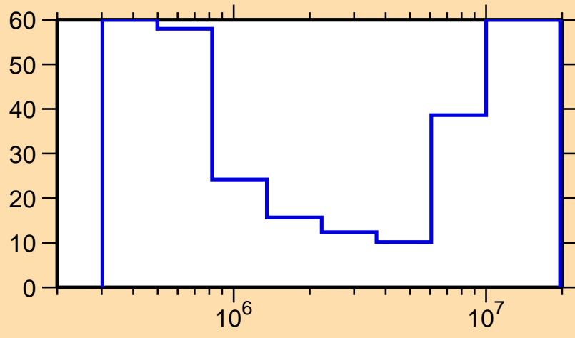
\Delta\sigma/\sigma vs. E for ^{144}\text{Ce}(n,\text{inel.})
