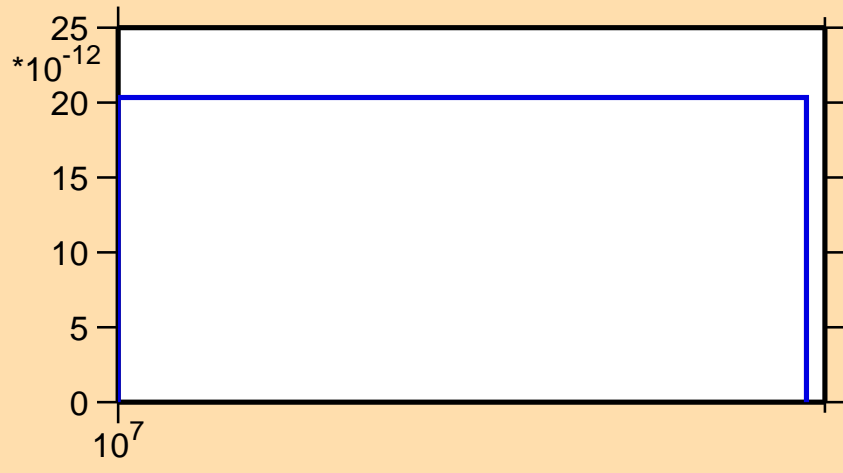
\sigma vs. E for ^{144}\text{Ce}(n,2np)
