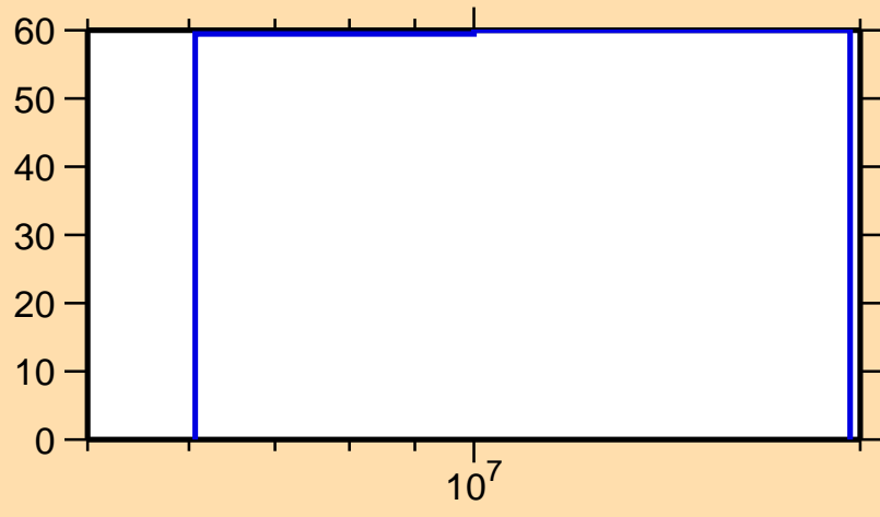
\Delta\sigma/\sigma vs. E for ^{144}\text{Ce}(n,n\text{cont.})
