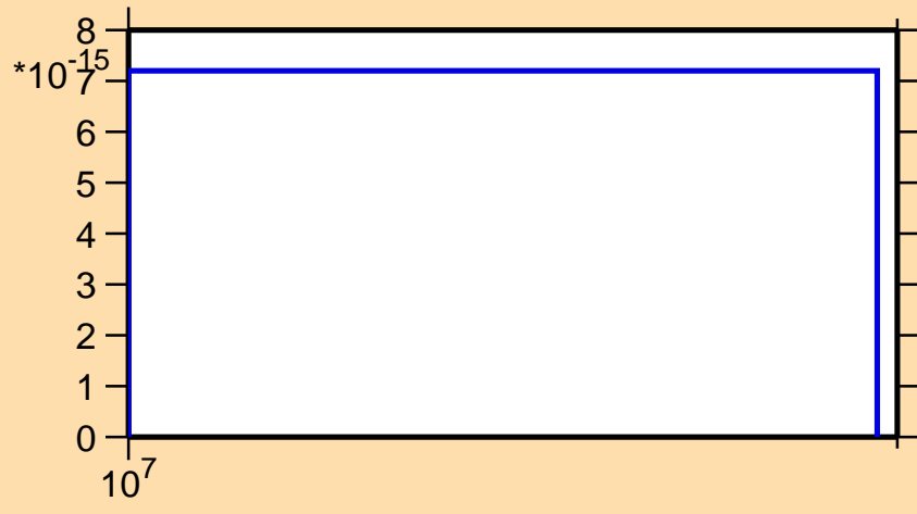
\sigma vs. E for ^{144}\text{Ce}(n,\text{He}3)
