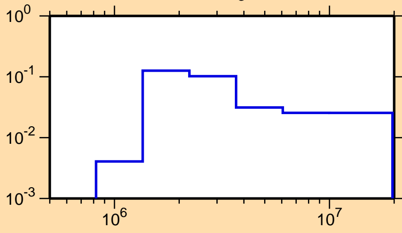
\sigma vs. E for ^{144}\text{Ce}(n,n_3)
