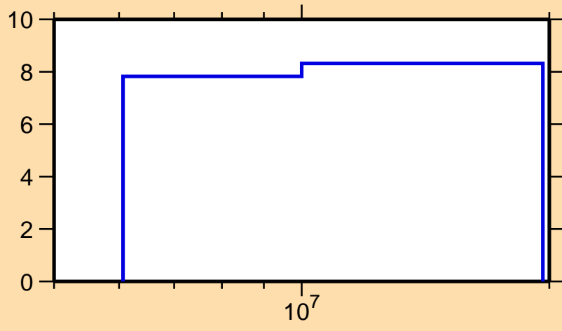
\Delta\sigma/\sigma vs. E for ^{144}\text{Ce}(n,\text{nonel.})
