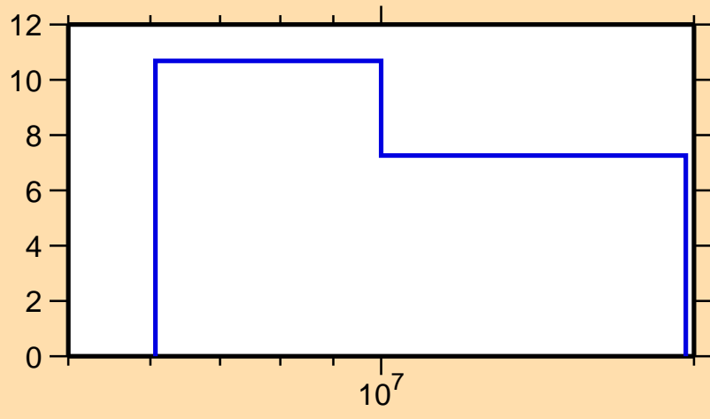
\Delta\sigma/\sigma vs. E for ^{144}\text{Ce}(n,\text{el.})
