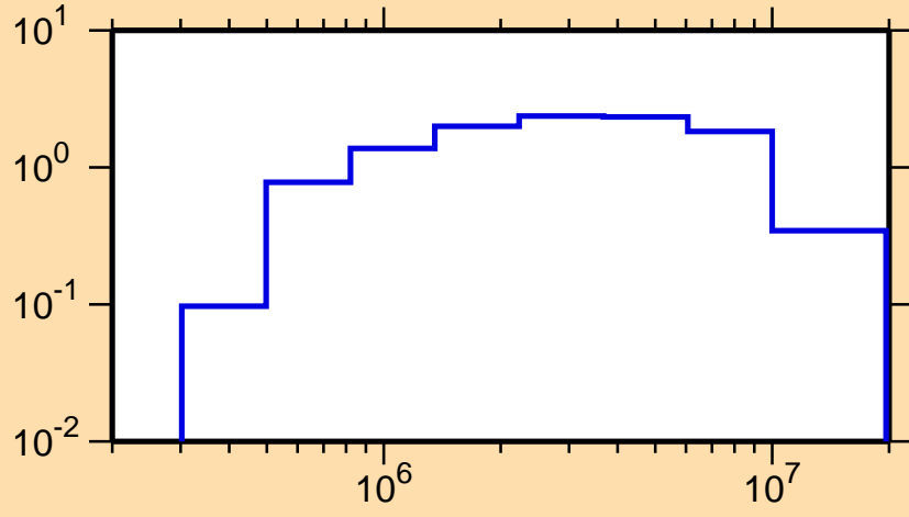
\sigma vs. E for ^{144}\text{Ce}(n,\text{inel.})
