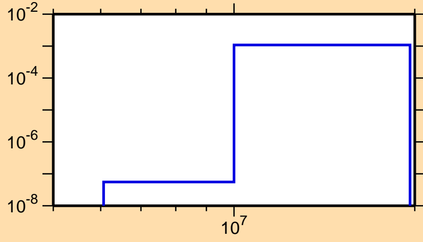
\sigma vs. E for ^{144}\text{Ce}(n,p)
