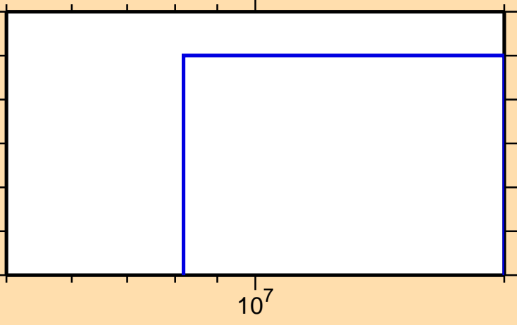
\sigma vs. E for ^{144}\text{Ce}(n,nt)
