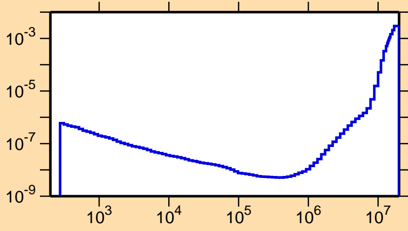
\sigma vs. E for ^{145}\text{Ce}(n,\alpha)
