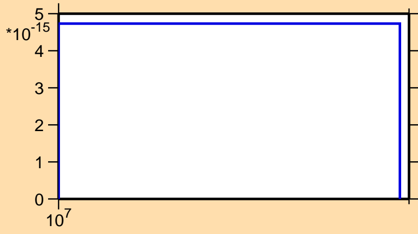
\sigma vs. E for ^{145}\text{Ce}(n,\text{He3})
