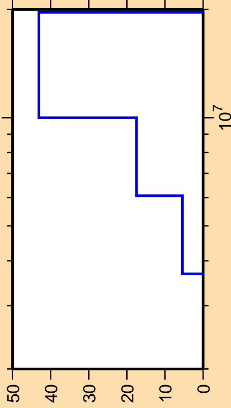
\Delta\sigma/\sigma vs. E for ^{145}\text{Ce}(n,n\text{cont.})
