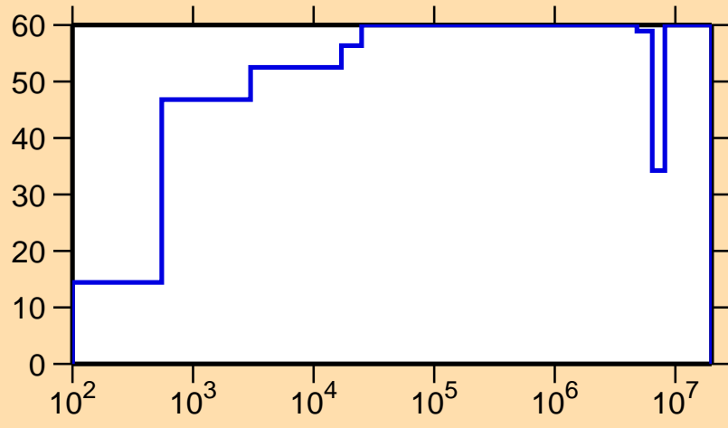
\Delta\sigma/\sigma vs. E for ^{145}\text{Ce}(n,\gamma)
