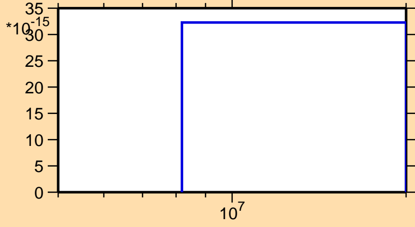
\sigma vs. E for ^{145}\text{Ce}(n,p\alpha)
