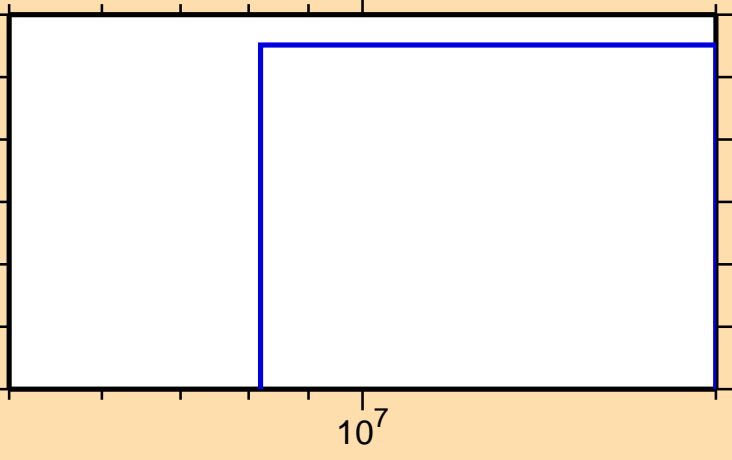
\sigma vs. E for ^{146}\text{Ce}(n,nt)
