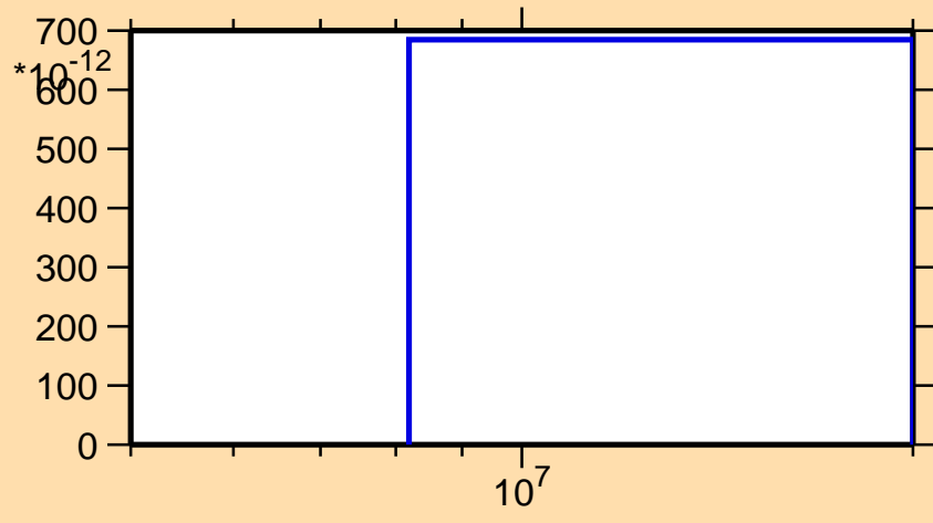
\sigma vs. E for ^{146}\text{Ce}(n,\text{nd})
