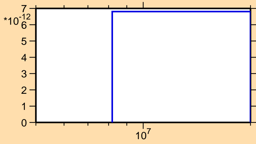
\sigma vs. E for ^{146}\text{Ce}(n,2np)
