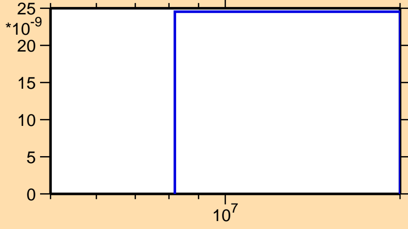
\sigma vs. E for ^{146}\text{Ce}(n,2n\alpha)
