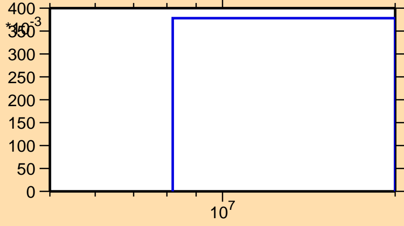
\sigma vs. E for ^{146}\text{Ce}(n,3n)
