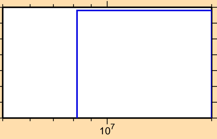
\sigma vs. E for ^{147}\text{Ce}(n,t)
