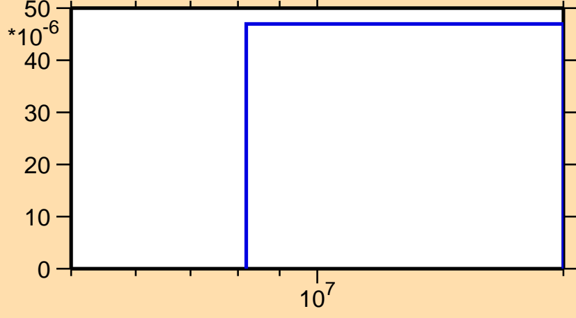
\sigma vs. E for ^{147}\text{Ce}(n,d)
