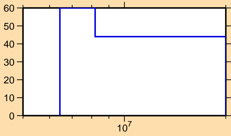
\Delta\sigma/\sigma vs. E for ^{147}\text{Ce}(n,n_1)
