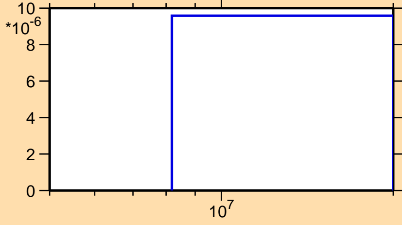
\sigma vs. E for ^{147}\text{Ce}(n,np)
