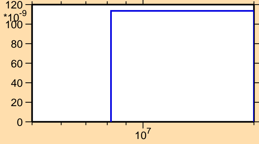
\sigma vs. E for ^{147}\text{Ce}(n,2n\alpha)
