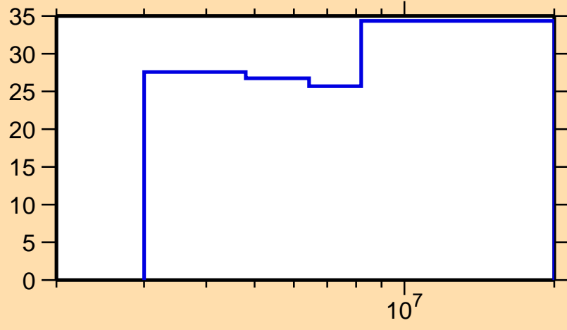
\Delta\sigma/\sigma vs. E for ^{147}\text{Ce}(n,2n)
