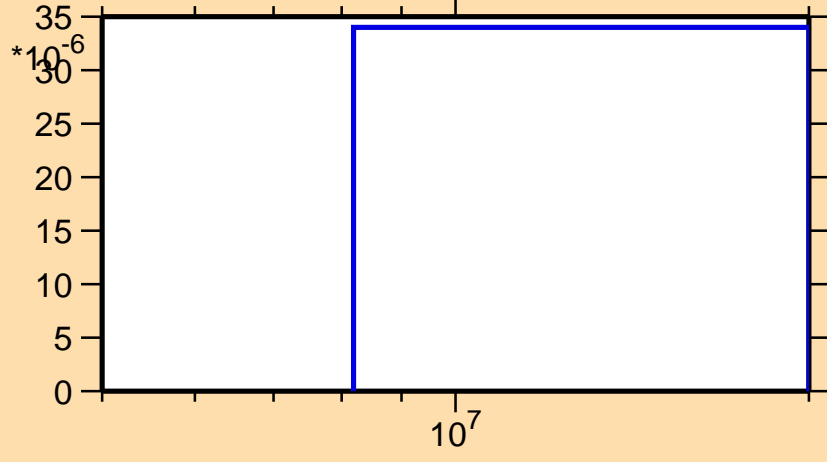
\sigma vs. E for ^{147}\text{Ce}(n,t)
