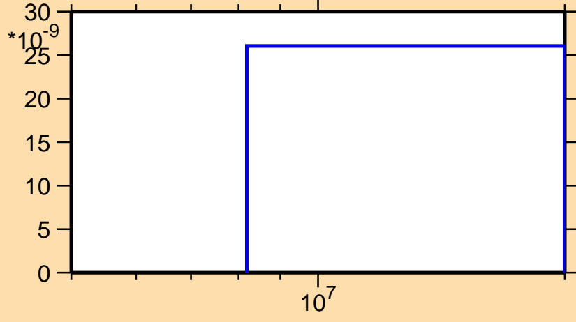
\sigma vs. E for ^{147}\text{Ce}(n,nt)
