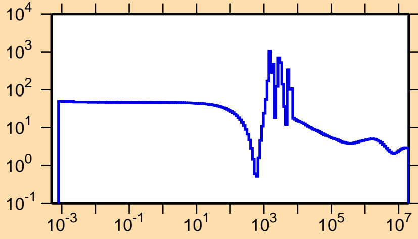
\sigma vs. E for ^{148}\text{Ce}(n,\text{el.})
