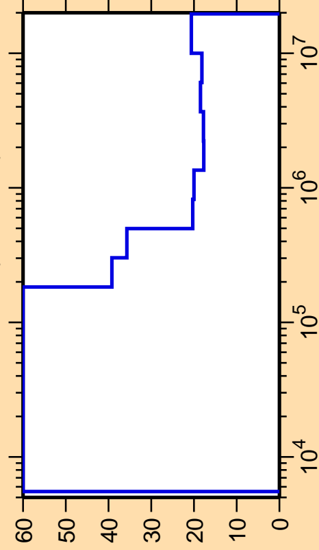
\Delta\sigma/\sigma vs. E for ^{148}\text{Ce}(n,\text{nonel.})
