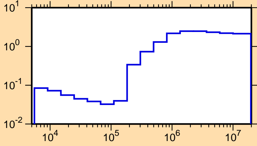
\sigma vs. E for ^{148}\text{Ce}(n,\text{nonel.})
