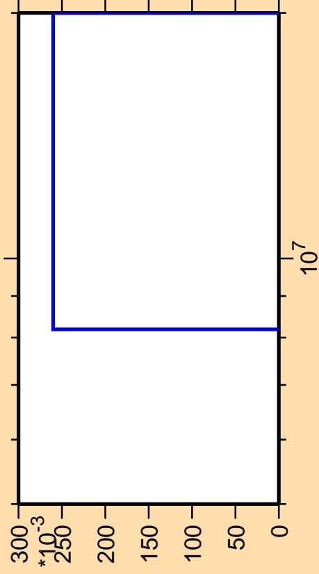
\Delta\sigma/\sigma vs. E for ^{148}\text{Ce}(n,2np)
