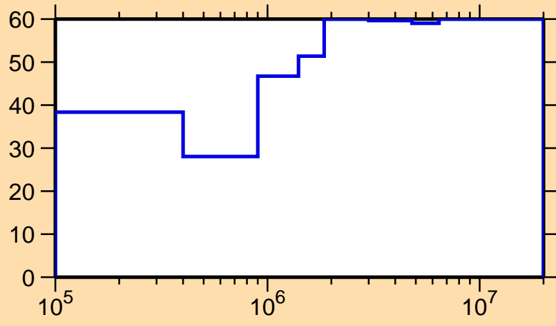
\Delta\sigma/\sigma vs. E for ^{148}\text{Ce}(n,n_1)
