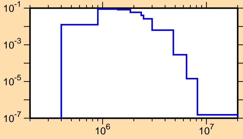
\sigma vs. E for ^{148}\text{Ce}(n,n_4)
