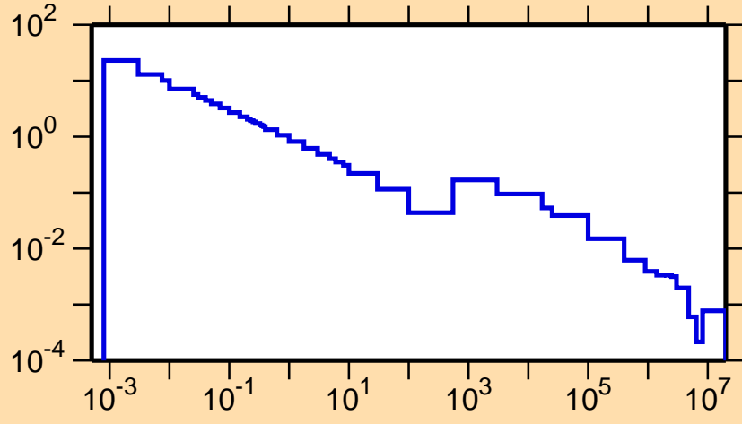
\sigma vs. E for ^{148}\text{Ce}(n,\gamma)
