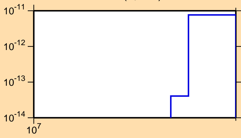
\sigma vs. E for ^{149}\text{Ce}(n,3n\alpha)
