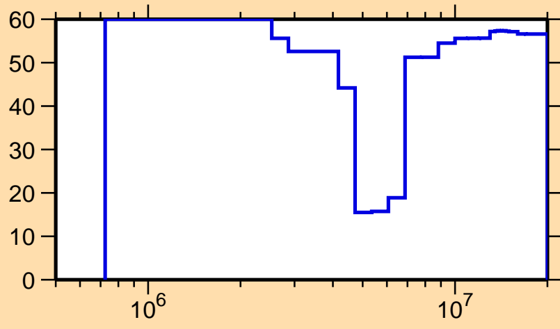
\Delta\sigma/\sigma vs. E for ^{149}\text{Ce}(n,n\text{cont.})
