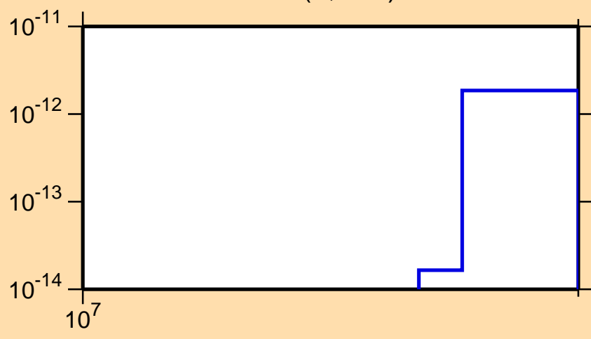
\sigma vs. E for ^{150}\text{Ce}(n,3n\alpha)
