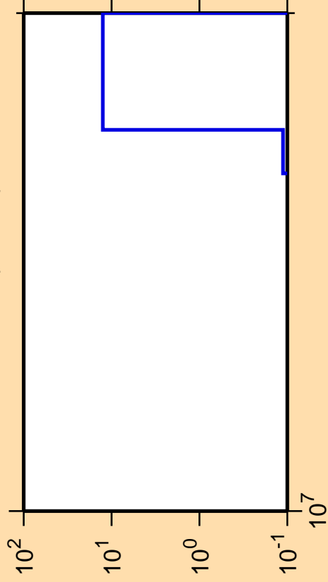
\Delta\sigma/\sigma vs. E for ^{150}\text{Ce}(n,3n\alpha)
