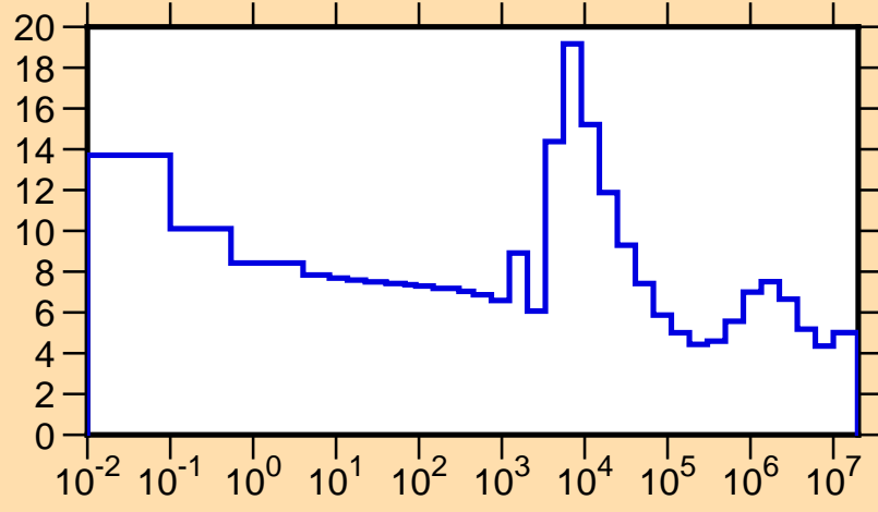
\sigma vs. E for ^{150}\text{Ce}(n,\text{tot.})
