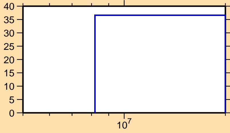
\Delta\sigma/\sigma vs. E for ^{150}\text{Ce}(n,n_1)
