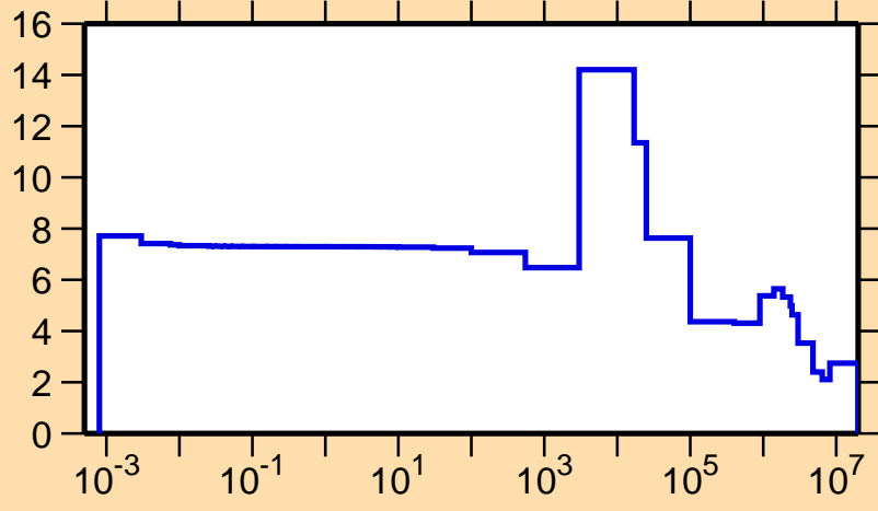
\sigma vs. E for ^{150}\text{Ce}(n,\text{el.})
