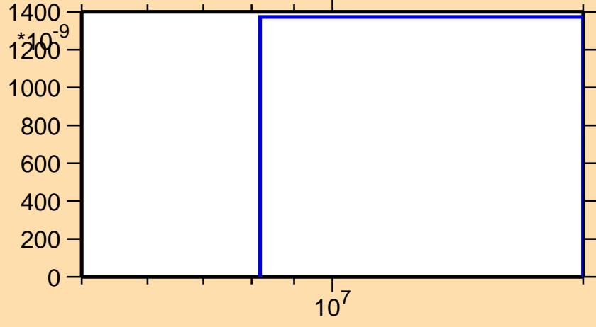
\sigma vs. E for ^{150}\text{Ce}(n,d)
