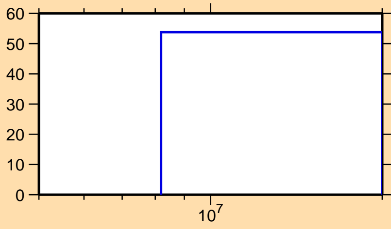
\Delta\sigma/\sigma vs. E for ^{150}\text{Ce}(n,ncont.)
