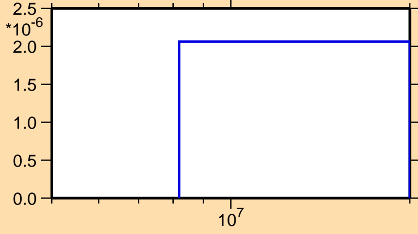
\sigma vs. E for ^{150}\text{Ce}(n,n\alpha)
