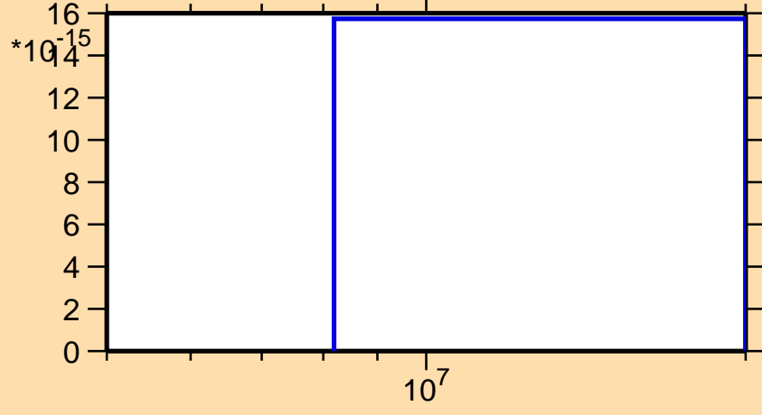
\sigma vs. E for ^{150}\text{Ce}(n,3n\alpha)
