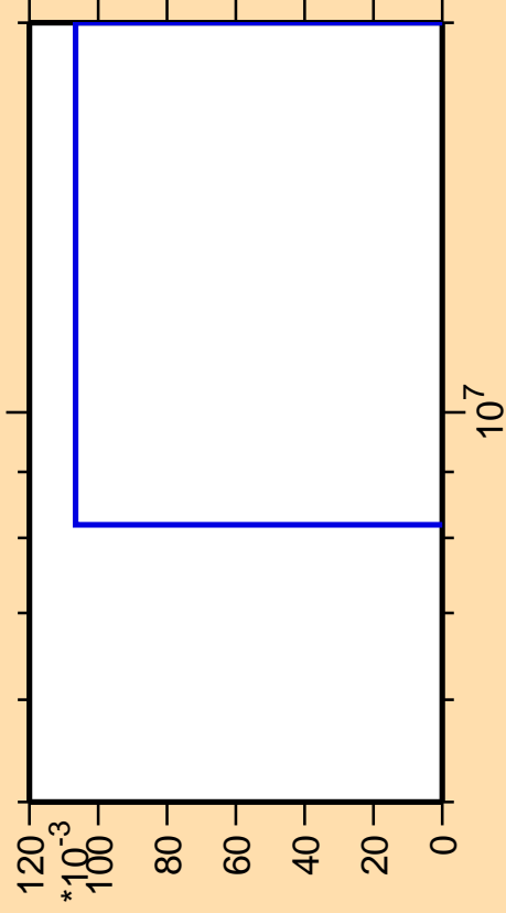
\Delta\sigma/\sigma vs. E for ^{150}\text{Ce}(n,3n\alpha)
