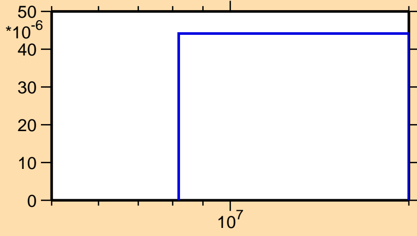
\sigma vs. E for ^{150}\text{Ce}(n,p)
