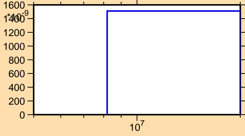
\sigma vs. E for ^{150}\text{Ce}(n,t)
