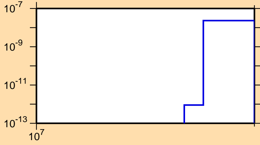
\sigma vs. E for ^{152}\text{Ce}(n,nt)
