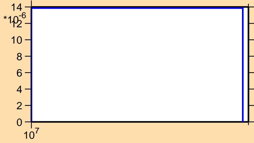
\sigma vs. E for ^{152}\text{Ce}(n,p)
