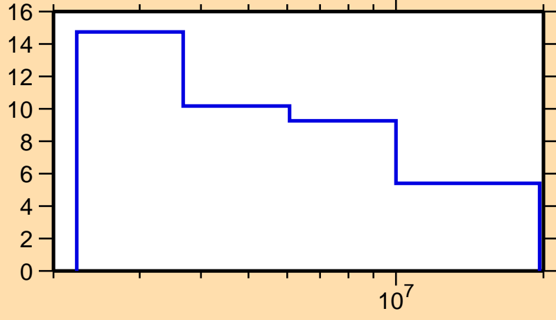
\Delta\sigma/\sigma vs. E for ^{152}\text{Ce}(n,n\text{onel.})
