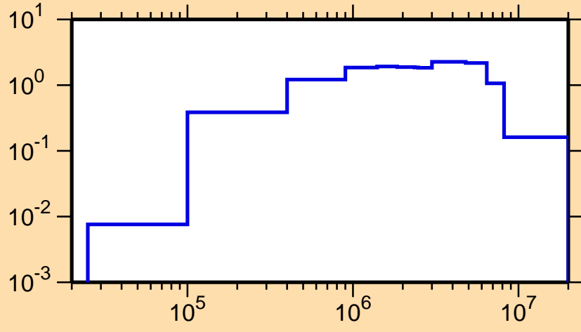
\sigma vs. E for ^{152}\text{Ce}(n,\text{inel.})
