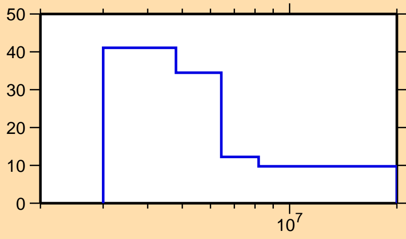
\Delta\sigma/\sigma vs. E for ^{152}\text{Ce}(n,\text{el.})
