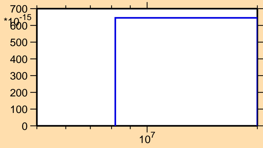
\sigma vs. E for ^{152}\text{Ce}(n,\text{nd})
