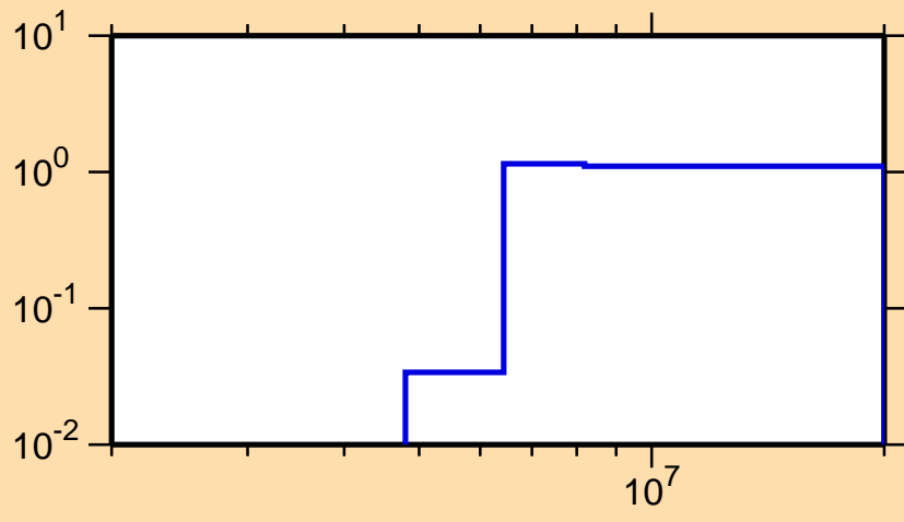
\sigma vs. E for ^{152}\text{Ce}(n,2n)
