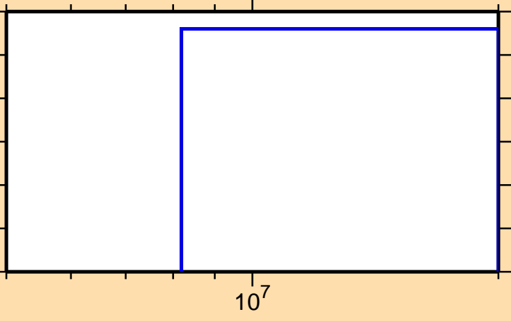
\sigma vs. E for ^{152}\text{Ce}(n,p)
