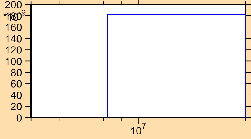
\sigma vs. E for ^{152}\text{Ce}(n,n\alpha)
