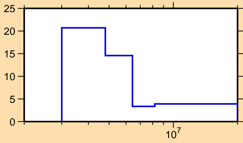
\Delta\sigma/\sigma vs. E for ^{152}\text{Ce}(n,\text{tot.})
