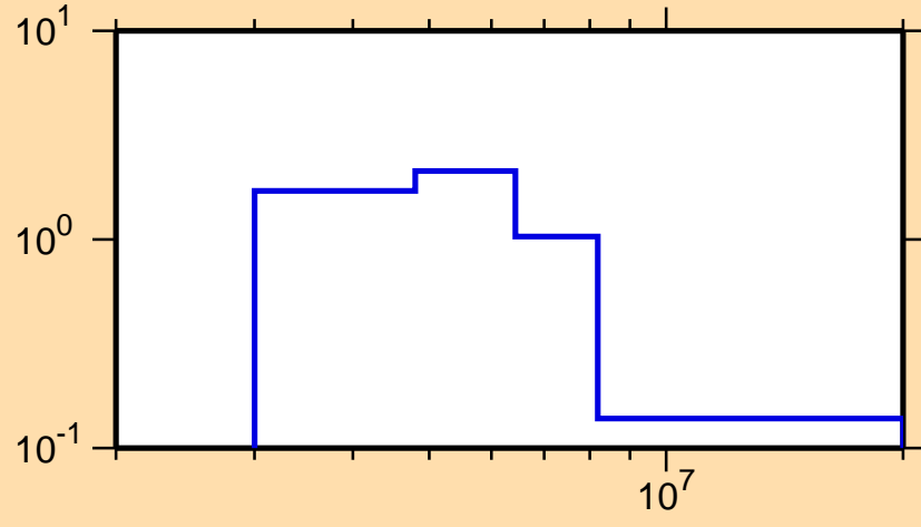
\sigma vs. E for ^{152}\text{Ce}(n,n\text{cont.})
