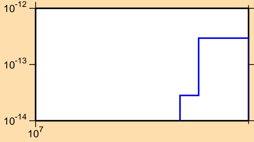
\sigma vs. E for ^{239}\text{Cf}(n,\text{pd})
