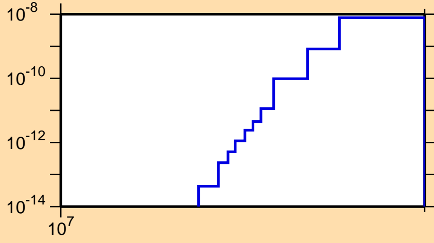
\sigma vs. E for ^{239}\text{Cf}(n,nd)
