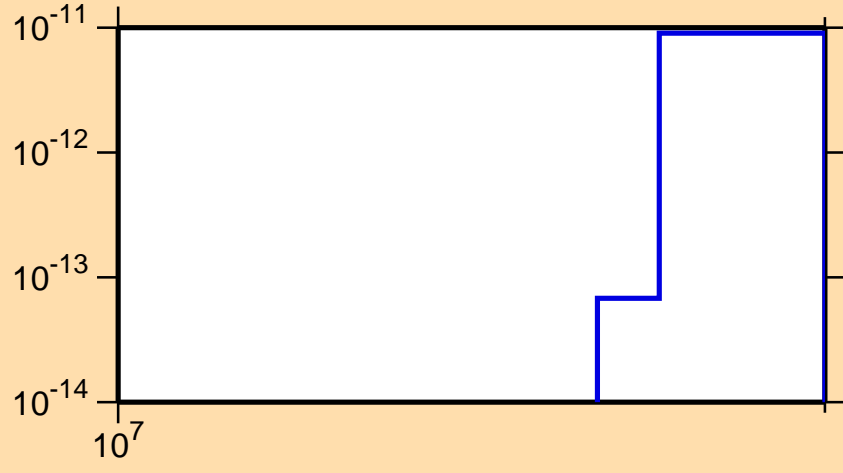
\sigma vs. E for ^{239}\text{Cf}(n,nt)
