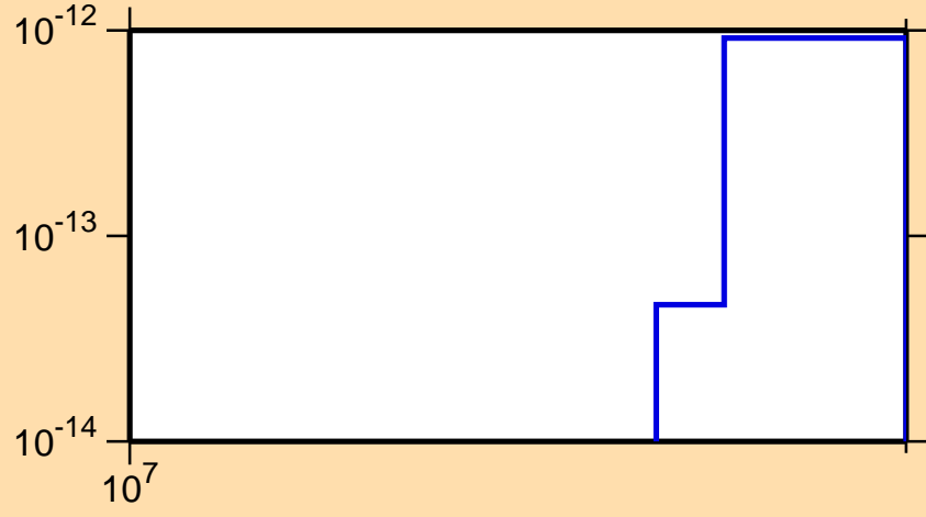
\sigma vs. E for ^{239}\text{Cf} (mt 34)
