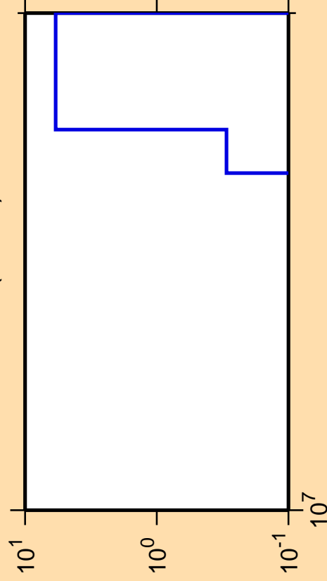
\Delta\sigma/\sigma vs. E for ^{239}\text{Cf} (mt 34)
