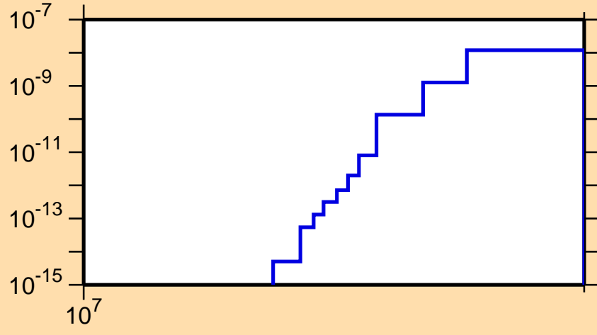
\sigma vs. E for ^{239}\text{Cf}(n,2np)
