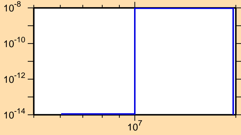
\sigma vs. E for ^{239}\text{Cf}(n,\text{He3})
