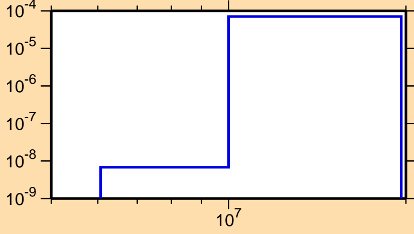
\sigma vs. E for ^{239}\text{Cf}(n,np)
