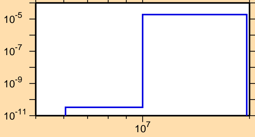
\sigma vs. E for ^{239}\text{Cf}(n,t)
