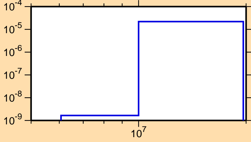
\sigma vs. E for ^{239}\text{Cf}(\text{mt } 45)
