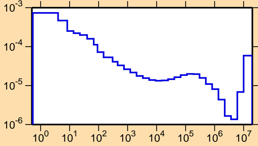
\sigma vs. E for ^{239}\text{Cf}(n,\alpha)
