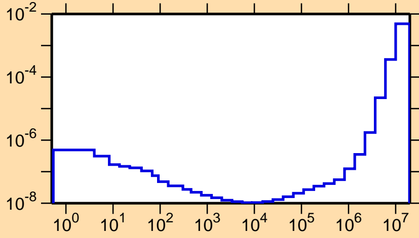
\sigma vs. E for ^{239}\text{Cf}(n,p\alpha)
