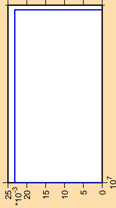
\Delta\sigma/\sigma vs. E for ^{239}\text{Cf}(n,\text{pd})
