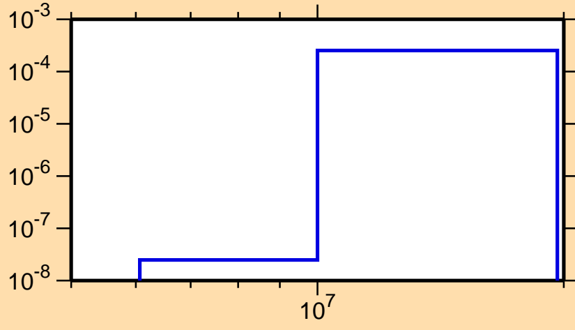
\sigma vs. E for ^{239}\text{Cf}(\text{mt117})
