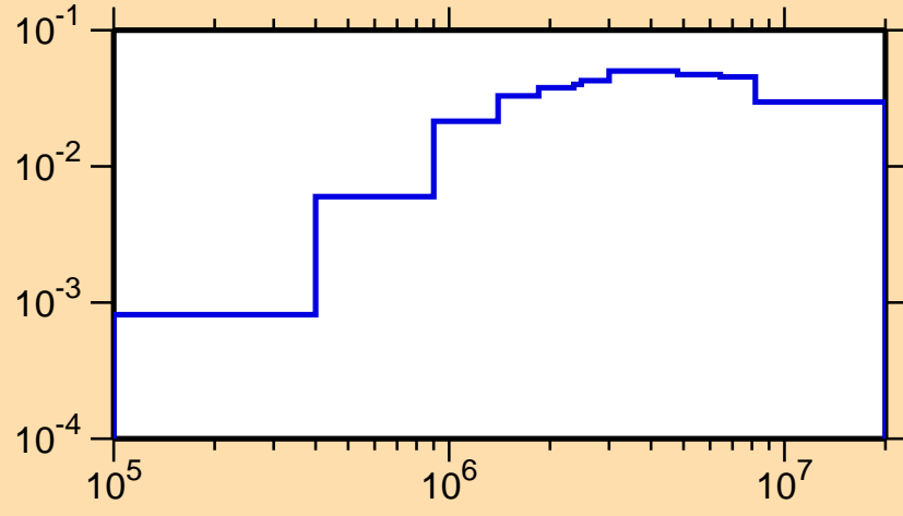
\sigma vs. E for ^{239}\text{Cf}(n,\text{inel.})
