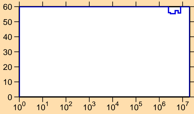
\Delta\sigma/\sigma vs. E for ^{239}\text{Cf}(n,p)
