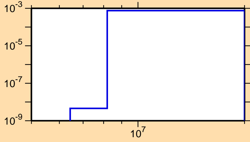
\sigma vs. E for ^{239}\text{Cf}(n,d)
