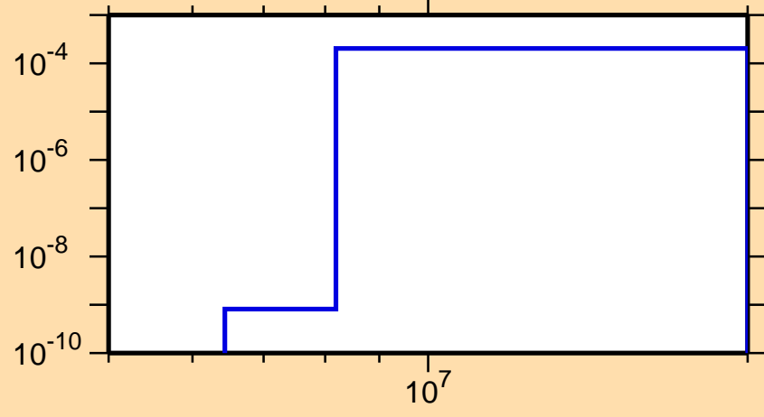
\sigma vs. E for ^{239}\text{Cf}(\text{mt117})
