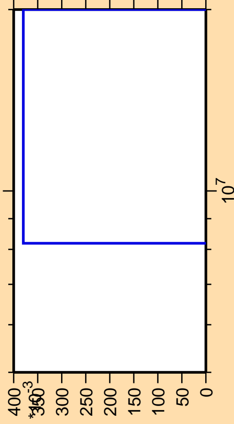
\Delta\sigma/\sigma vs. E for ^{239}\text{Cf}(n,nt)
