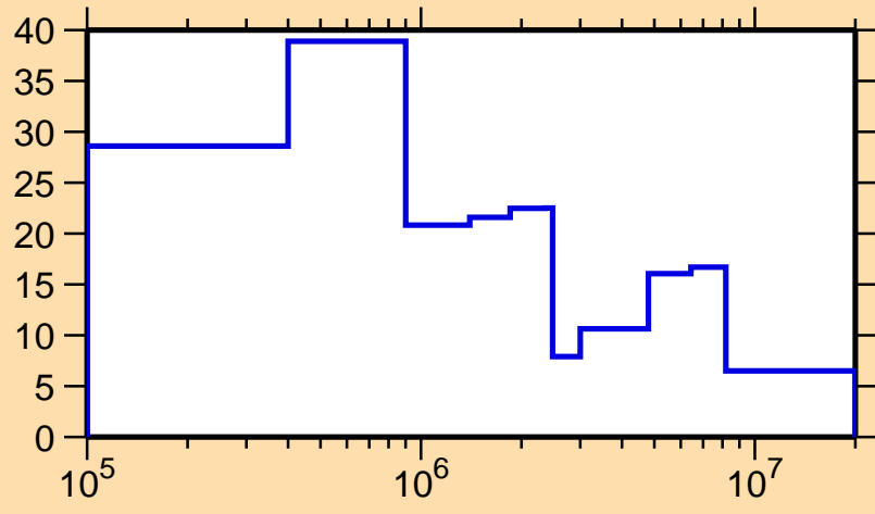
\Delta\sigma/\sigma vs. E for ^{239}\text{Cf}(n,\text{tot.})
