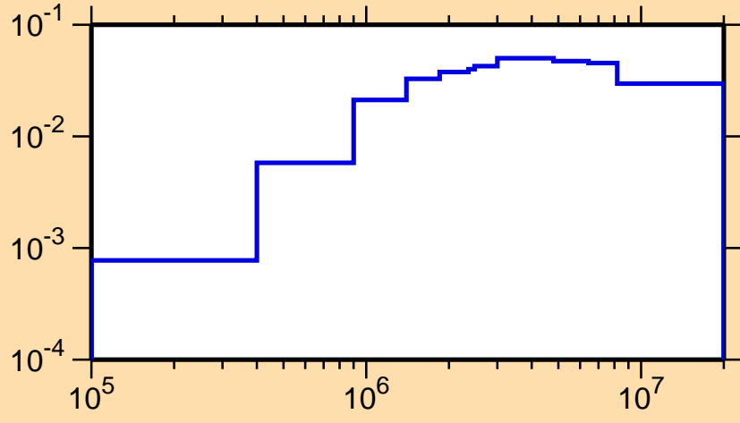
\sigma vs. E for ^{239}\text{Cf}(n,n\text{cont.})
