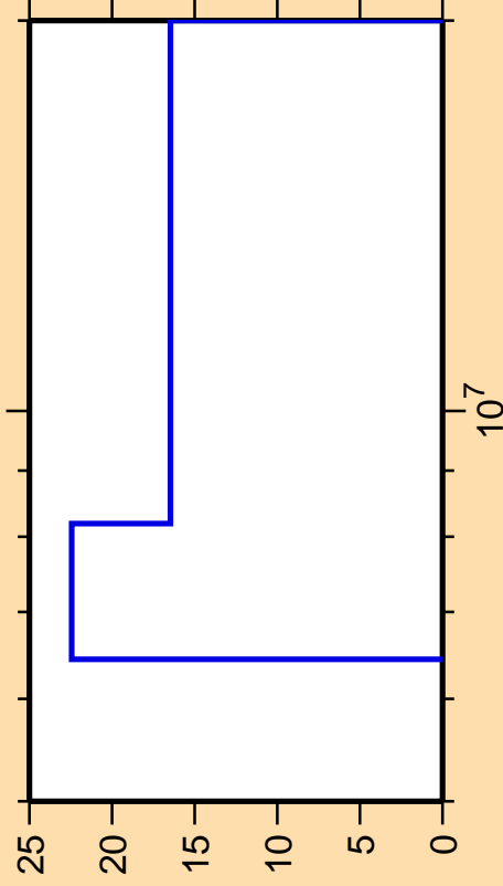
\Delta\sigma/\sigma vs. E for ^{239}\text{Cf}(n,f)
