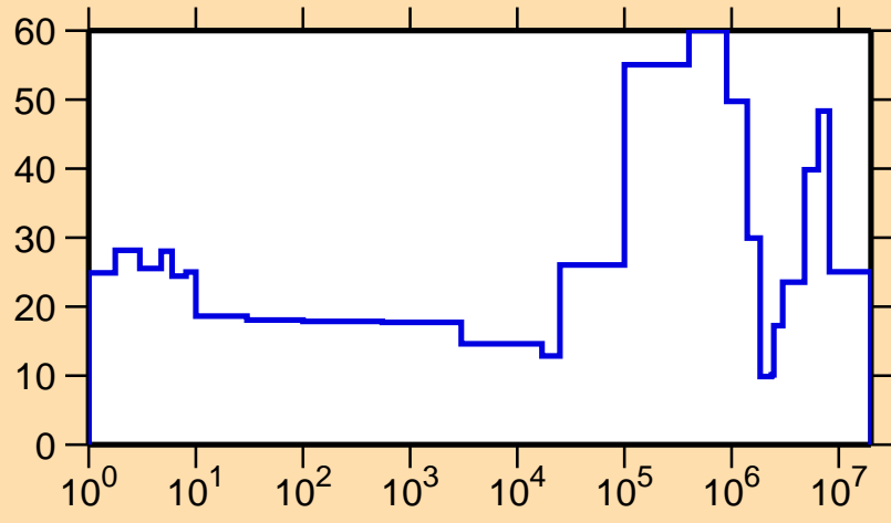
\Delta\sigma/\sigma vs. E for ^{239}\text{Cf}(n,\text{el.})
