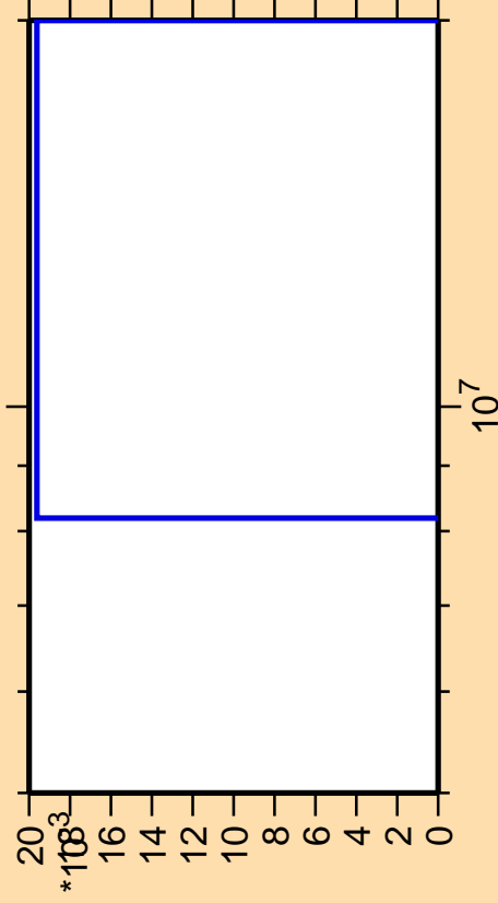
\Delta\sigma/\sigma vs. E for ^{239}\text{Cf}(n,pd)
