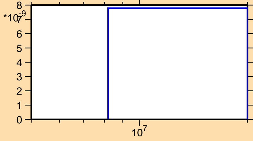
\sigma vs. E for ^{239}\text{Cf}(n,\text{He3})
