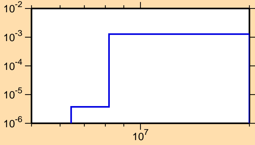
\sigma vs. E for ^{239}\text{Cf}(n,2n\alpha)
