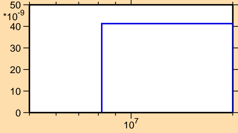
\sigma vs. E for ^{239}\text{Cf}(n,3n)
