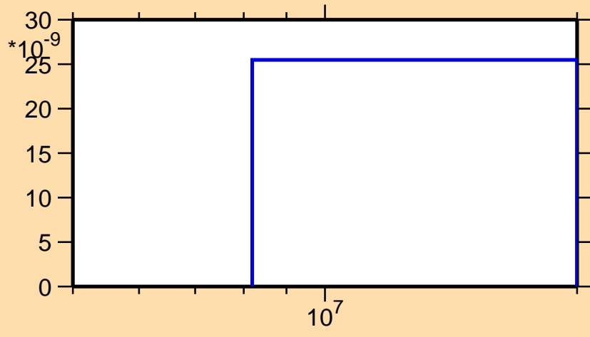
\sigma vs. E for ^{239}\text{Cf}(n,3n\alpha)
