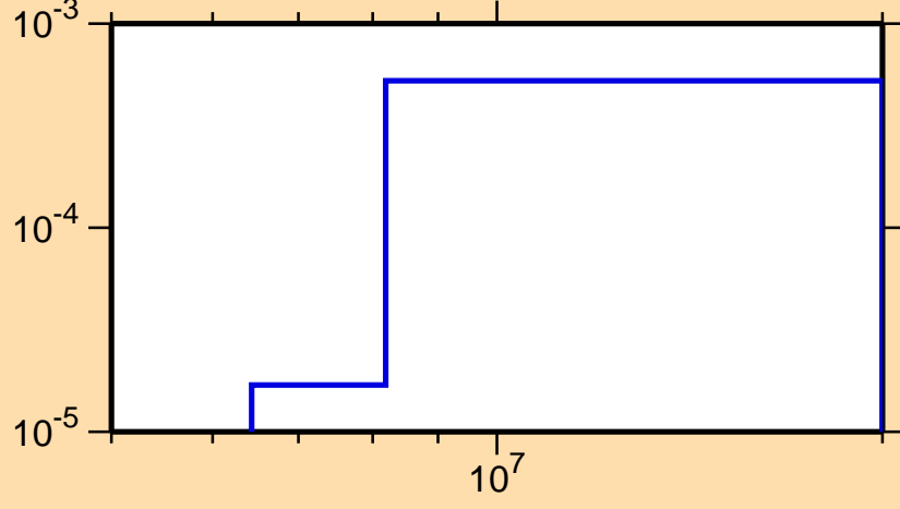
\sigma vs. E for ^{239}\text{Cf}(n,2n)
