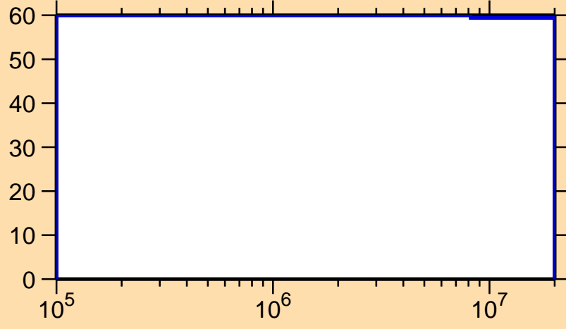
\Delta\sigma/\sigma vs. E for ^{239}\text{Cf}(n,n_1)
