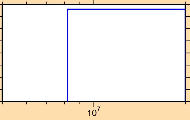
\sigma vs. E for ^{239}\text{Cf}(n,t)
