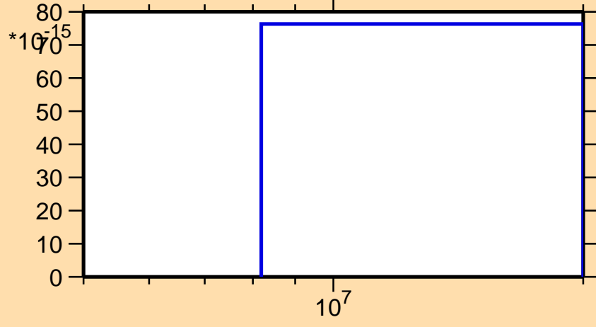
\sigma vs. E for ^{239}\text{Cf}(n,nt)
