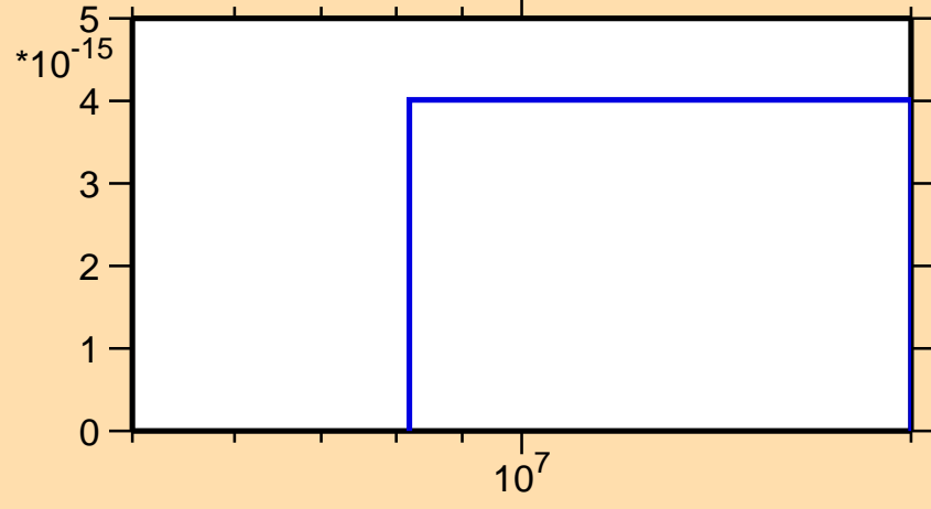
\sigma vs. E for ^{239}\text{Cf}(n,pd)
