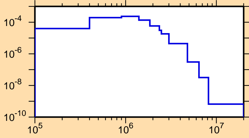
\sigma vs. E for ^{239}\text{Cf}(n,n_1)
