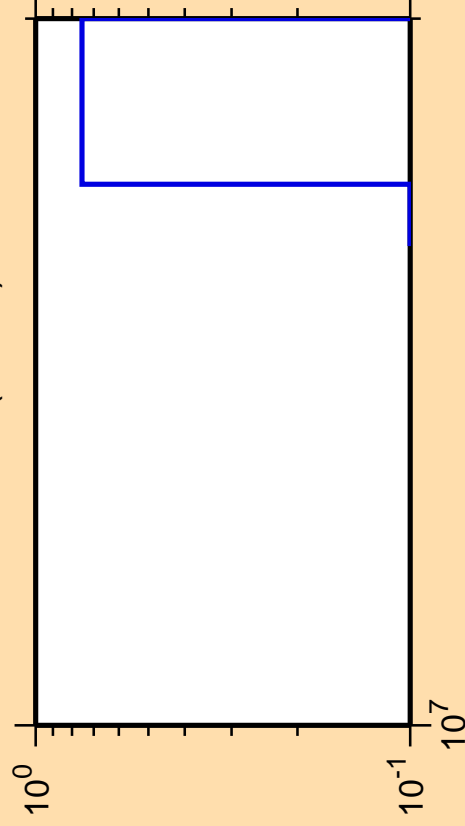
\Delta\sigma/\sigma vs. E for ^{240}\text{Cf}(\text{mt 34})
