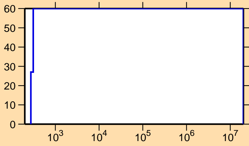
\Delta\sigma/\sigma vs. E for ^{240}\text{Cf}(n,p)
