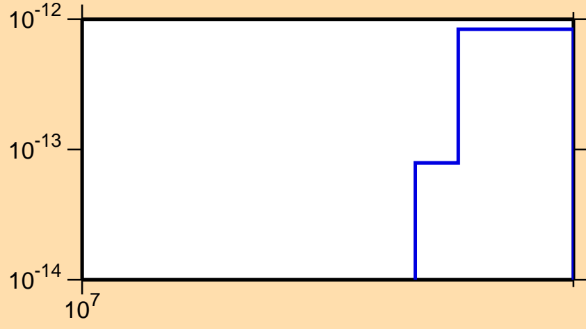
\sigma vs. E for ^{240}\text{Cf}(n,\text{pd})
