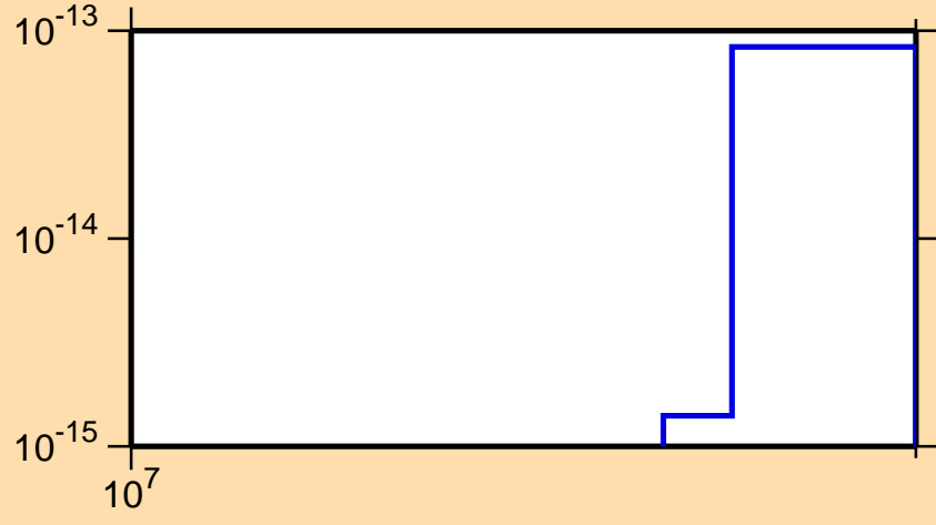
\sigma vs. E for ^{240}\text{Cf}(\text{mt 34})
