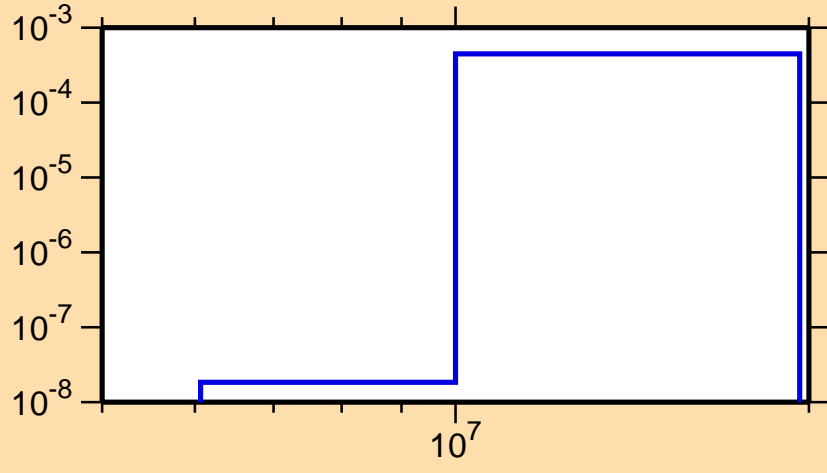
\sigma vs. E for ^{240}\text{Cf}(n,d)
