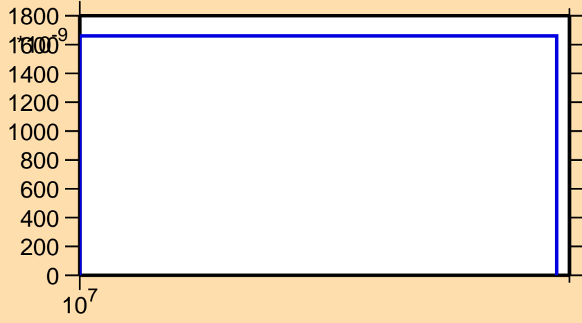
\sigma vs. E for ^{240}\text{Cf}(n,3n)
