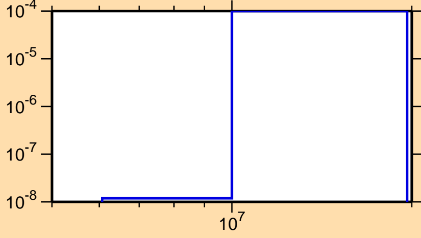
\sigma vs. E for ^{240}\text{Cf}(\text{mt } 45)
