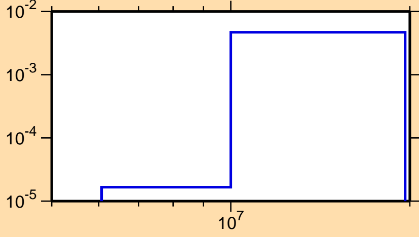
\sigma vs. E for ^{240}\text{Cf}(n,2n\alpha)
