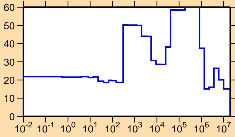
\Delta\sigma/\sigma vs. E for ^{240}\text{Cf}(n,\text{el.})
