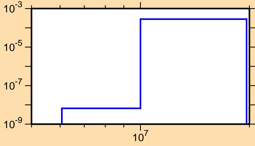
\sigma vs. E for ^{240}\text{Cf}(\text{mt117})
