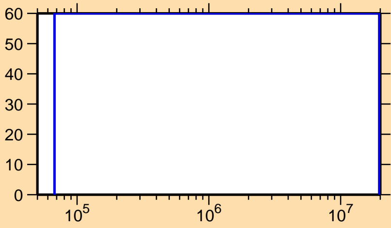
\Delta\sigma/\sigma vs. E for ^{240}\text{Cf}(n,\text{inel.})
