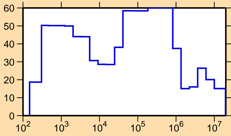
\Delta\sigma/\sigma vs. E for ^{240}\text{Cf}(n,el.)
