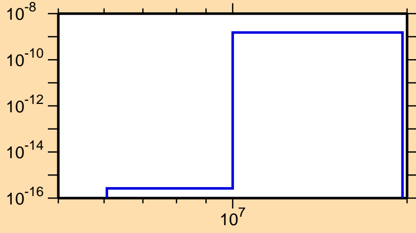
\sigma vs. E for ^{240}\text{Cf}(n,\text{He3})
