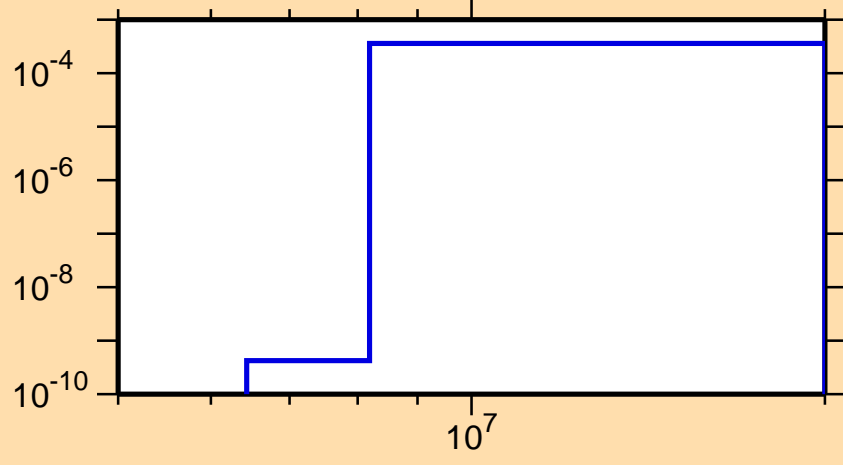
\sigma vs. E for ^{240}\text{Cf}(n,d)
