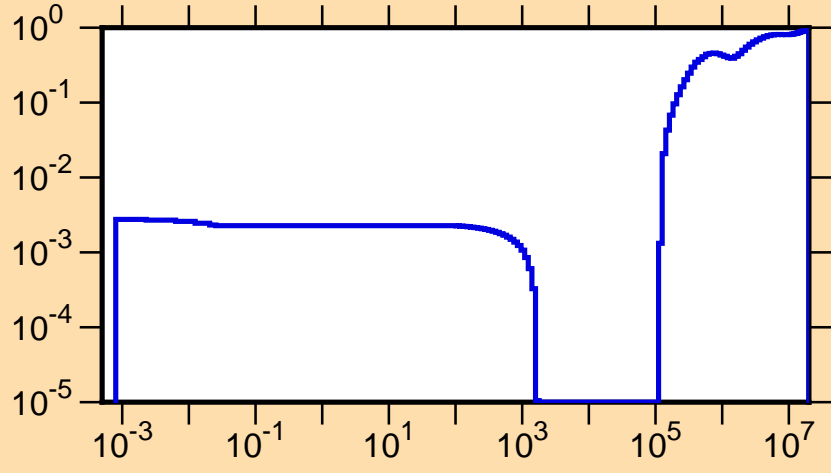
\mu vs. E for ^{241}\text{Cf}(\text{mt251})
