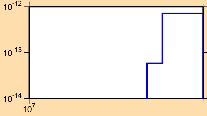
\sigma vs. E for ^{241}\text{Cf}(n,\text{pd})
