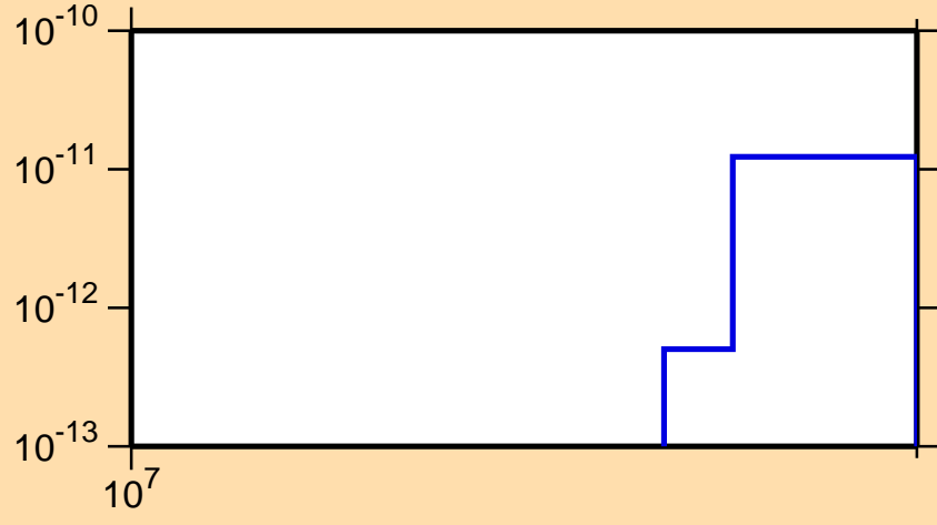
\sigma vs. E for ^{241}\text{Cf}(\text{mt } 34)
