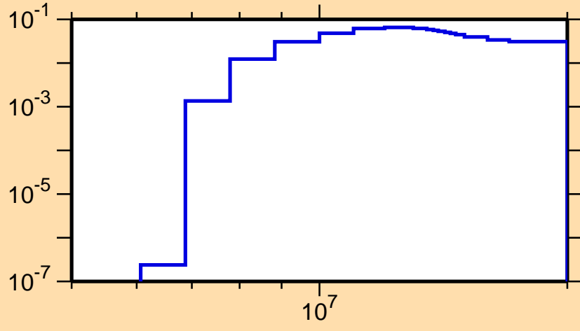
\sigma vs. E for ^{241}\text{Cf}(n,2n\alpha)
