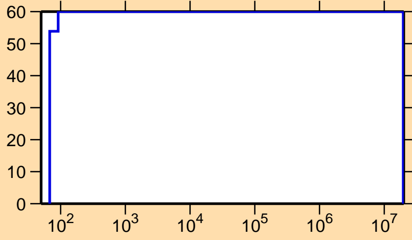
\Delta\sigma/\sigma vs. E for ^{241}\text{Cf}(n,\gamma)
