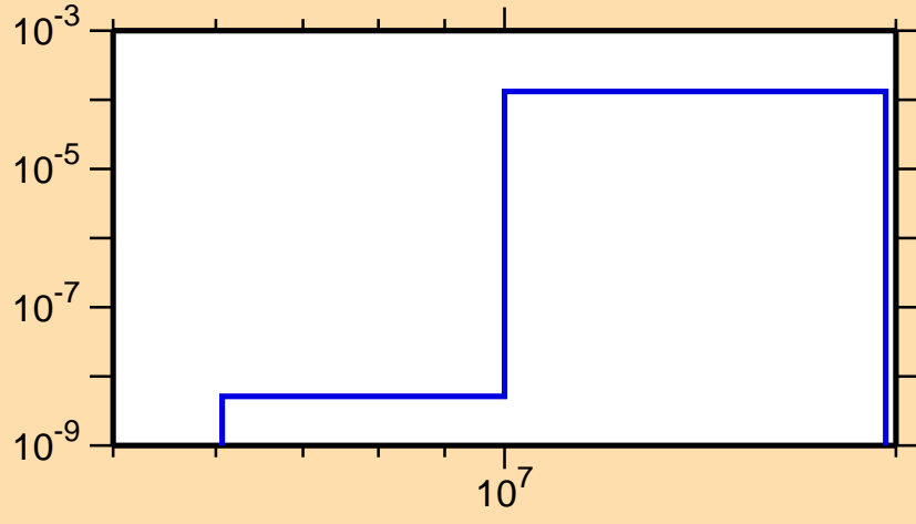
\sigma vs. E for ^{241}\text{Cf}(\text{mt117})
