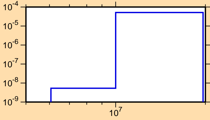
\sigma vs. E for ^{241}\text{Cf}(\text{mt } 45)
