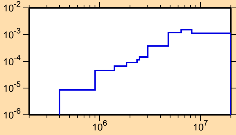
\sigma vs. E for ^{241}\text{Cf}(n,n\alpha)
