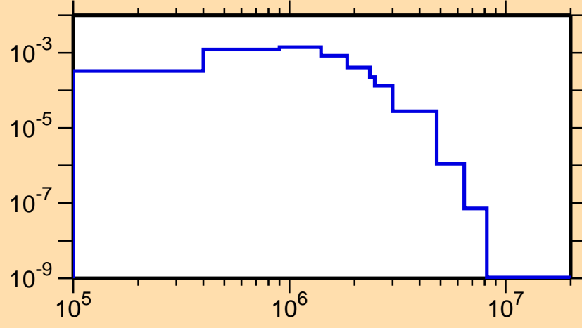
\sigma vs. E for ^{241}\text{Cf}(n,n_1)
