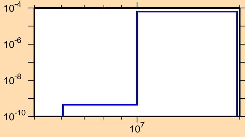
\sigma vs. E for ^{242}\text{Cf}(\text{mt117})
