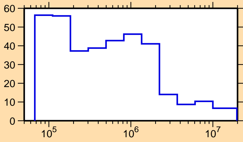
\Delta\sigma/\sigma vs. E for ^{242}\text{Cf}(n,\text{nonel.})
