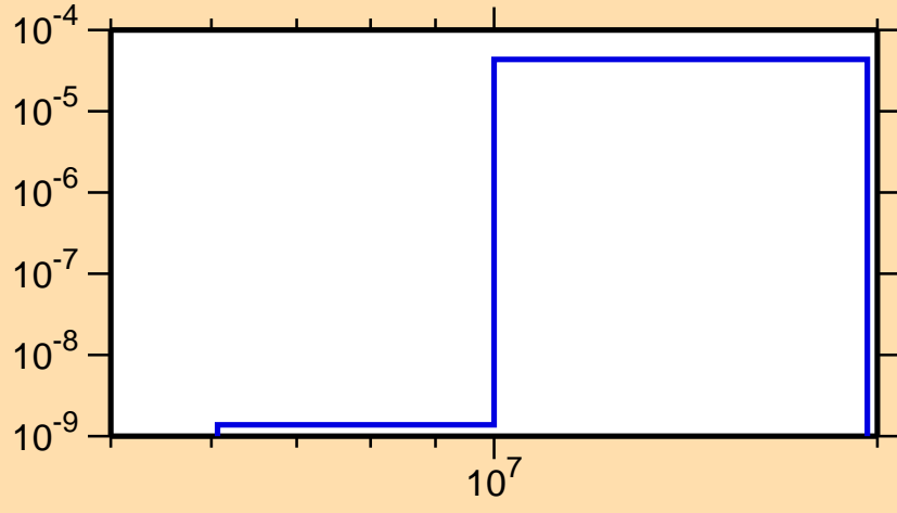
\sigma vs. E for ^{242}\text{Cf}(\text{mt } 45)
