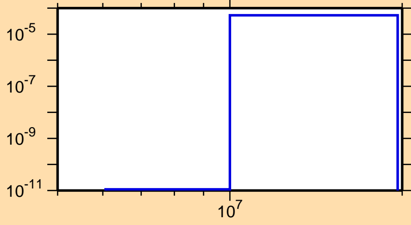
\sigma vs. E for ^{242}\text{Cf}(n,t)
