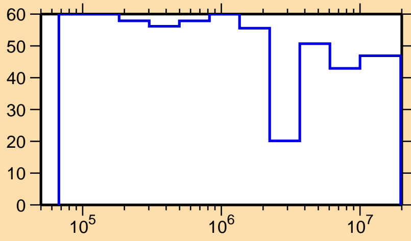
\Delta\sigma/\sigma vs. E for ^{242}\text{Cf}(n,n_1)
