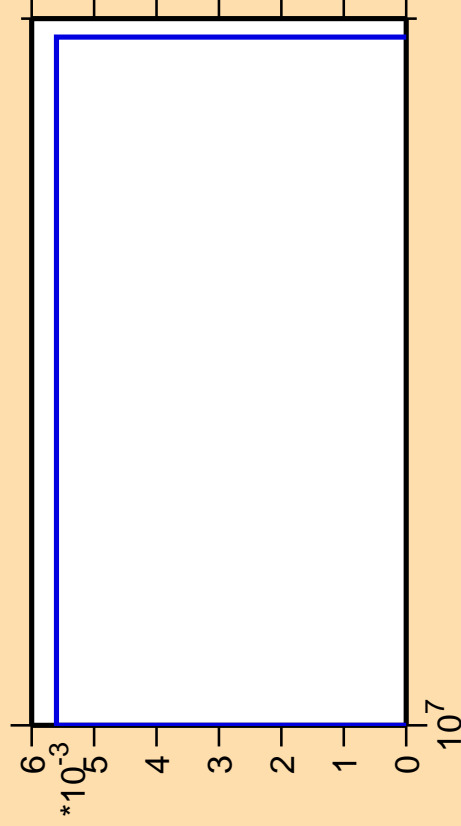
\Delta\sigma/\sigma vs. E for ^{242}\text{Cf}(\text{mt 34})
