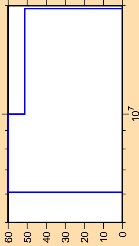
\Delta\sigma/\sigma vs. E for ^{242}\text{Cf}(\text{mt } 45)
