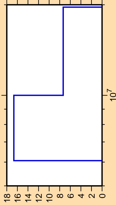
\Delta\sigma/\sigma vs. E for ^{242}\text{Cf}(n,f)
