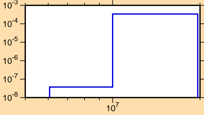
\sigma vs. E for ^{242}\text{Cf}(n,np)
