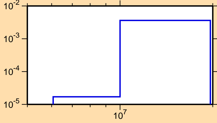
\sigma vs. E for ^{242}\text{Cf}(n,2n\alpha)
