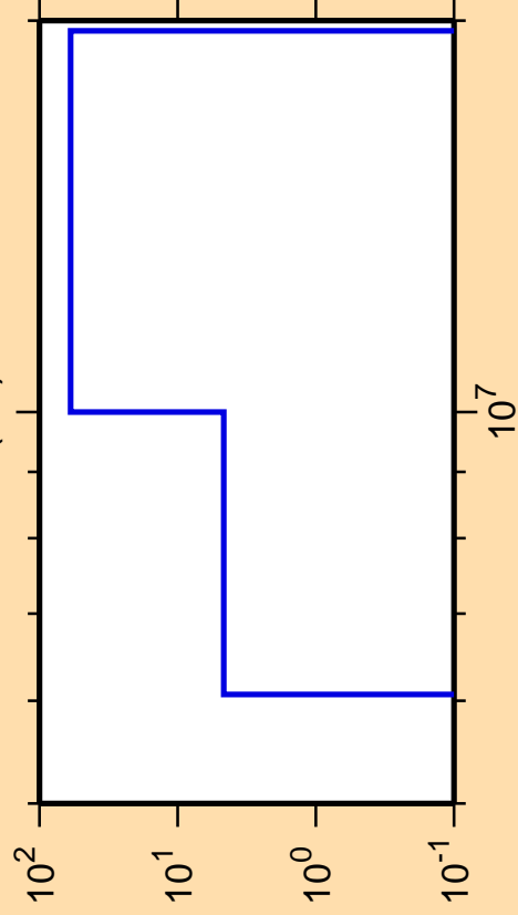
\Delta\sigma/\sigma vs. E for ^{242}\text{Cf}(n,t)
