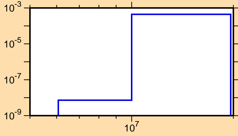
\sigma vs. E for ^{242}\text{Cf}(n,d)
