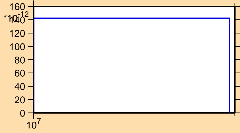
\sigma vs. E for ^{242}\text{Cf}(n,nt)
