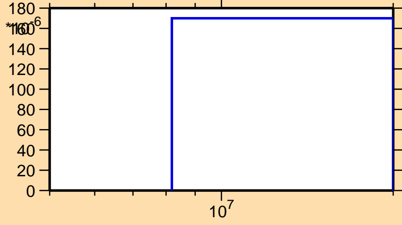
\sigma vs. E for ^{242}\text{Cf}(n,3n)
