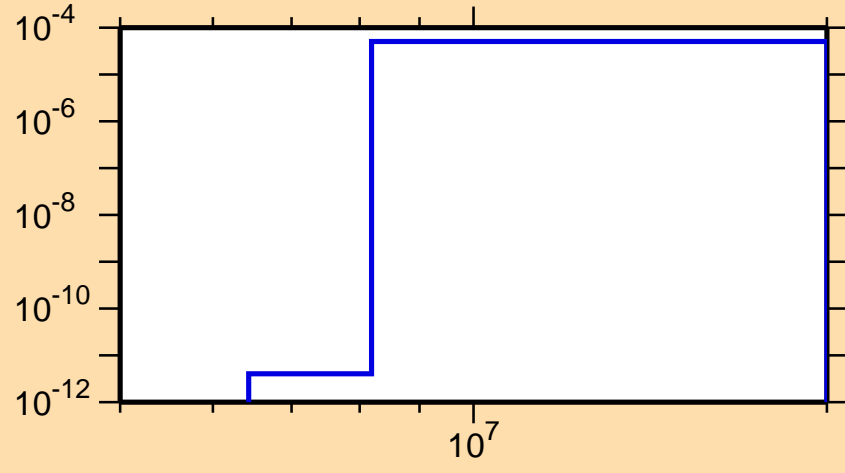
\sigma vs. E for ^{242}\text{Cf}(\text{mt117})
