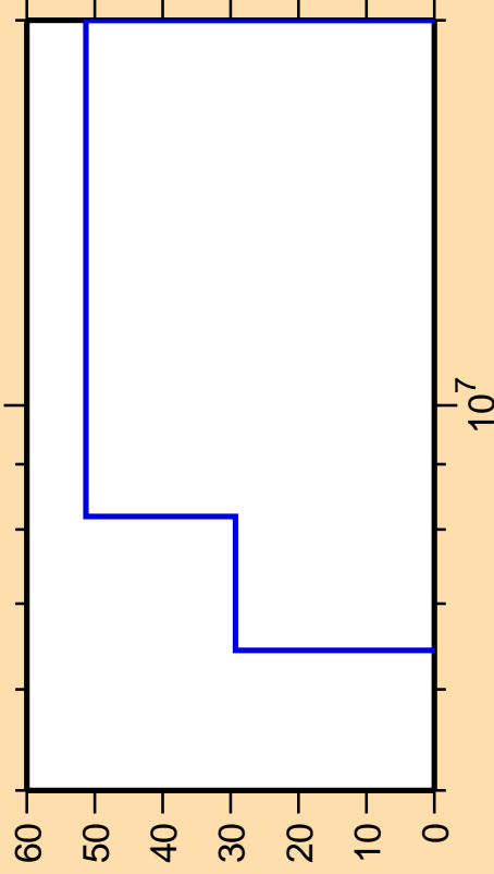
\Delta\sigma/\sigma vs. E for ^{242}\text{Cf}(\text{mt } 45)
