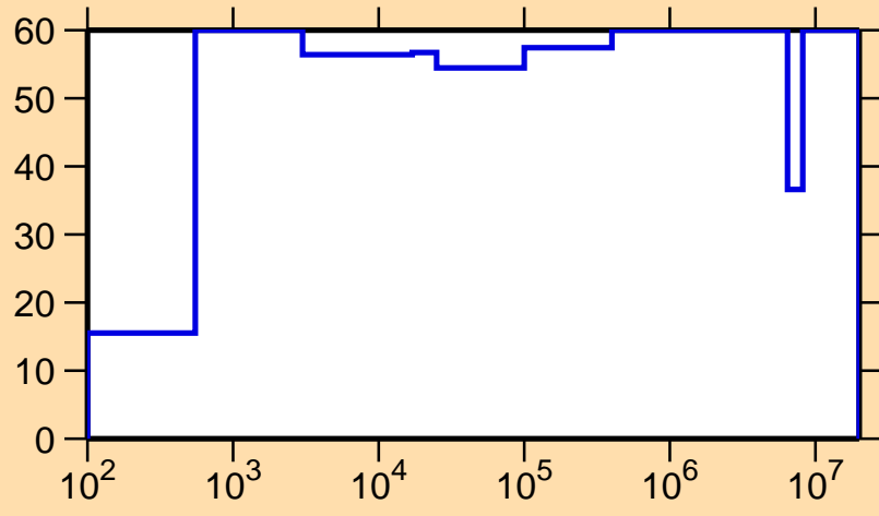
\Delta\sigma/\sigma vs. E for ^{242}\text{Cf}(n,\gamma)
