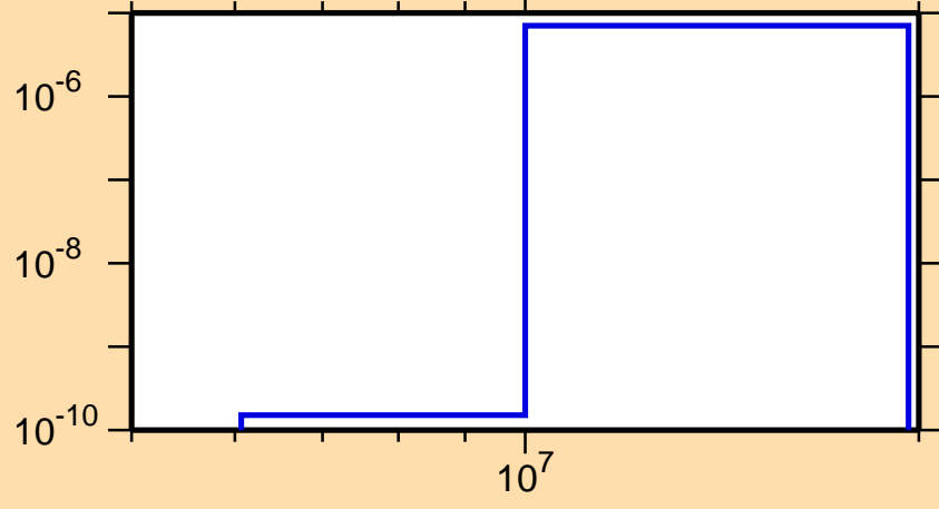
\sigma vs. E for ^{243}\text{Cf}(\text{mt117})
