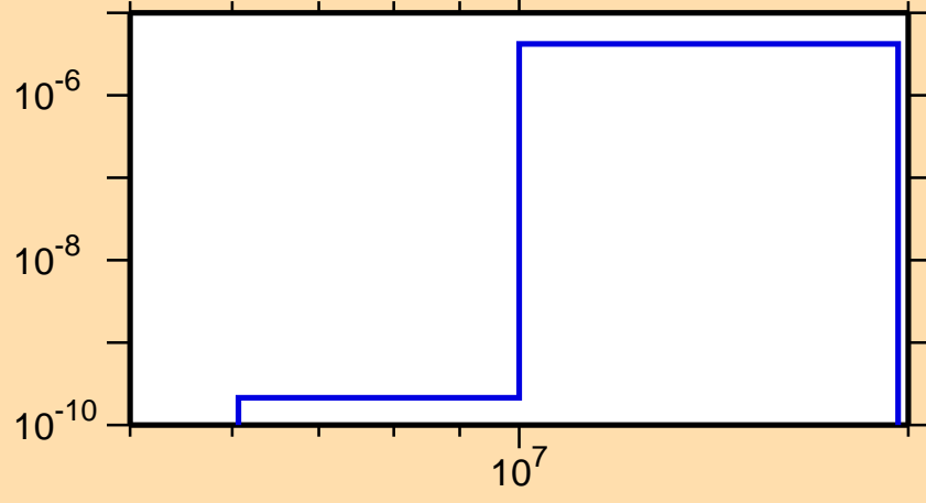
\sigma vs. E for ^{243}\text{Cf}(\text{mt } 45)
