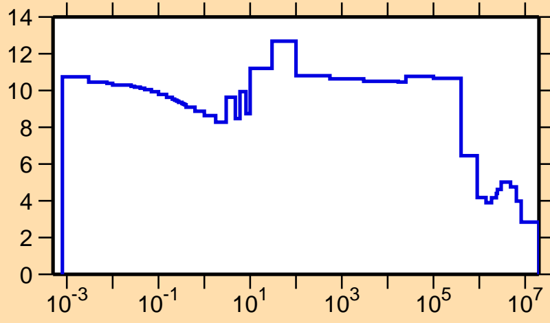
\sigma vs. E for ^{243}\text{Cf}(n,\text{el.})
