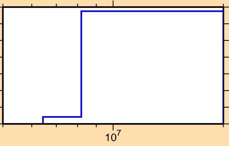
\sigma vs. E for ^{243}\text{Cf}(\text{mt117})
