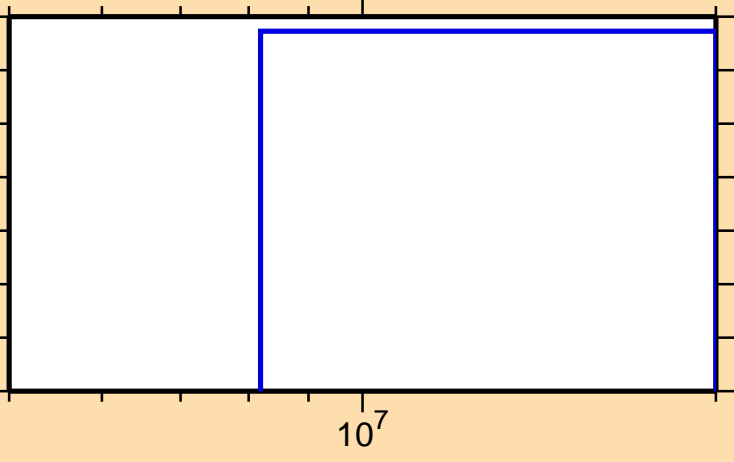
\sigma vs. E for ^{243}\text{Cf}(n,\text{He3})
