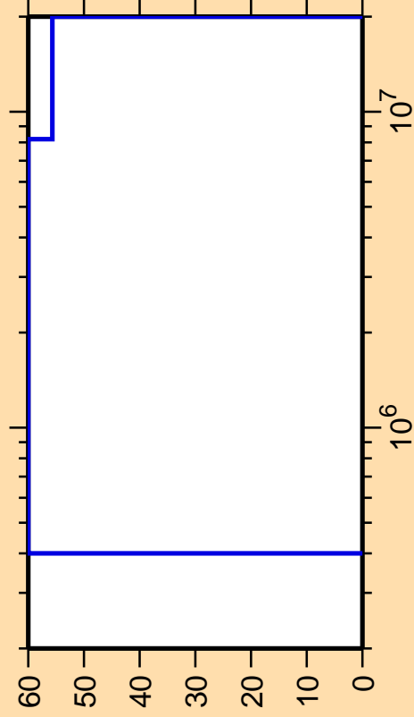
\Delta\sigma/\sigma vs. E for ^{243}\text{Cf}(n,ncont.)
