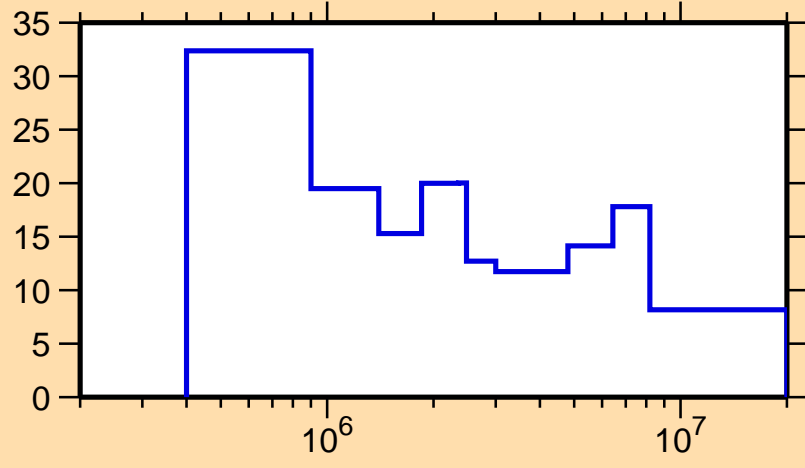
\Delta\sigma/\sigma vs. E for ^{243}\text{Cf}(n,el.)
