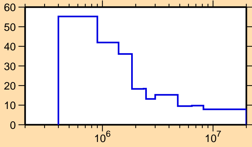
\Delta\sigma/\sigma vs. E for ^{243}\text{Cf}(n,n\text{onel.})
