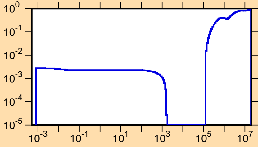
\mu vs. E for ^{244}\text{Cf}(\text{mt251})
