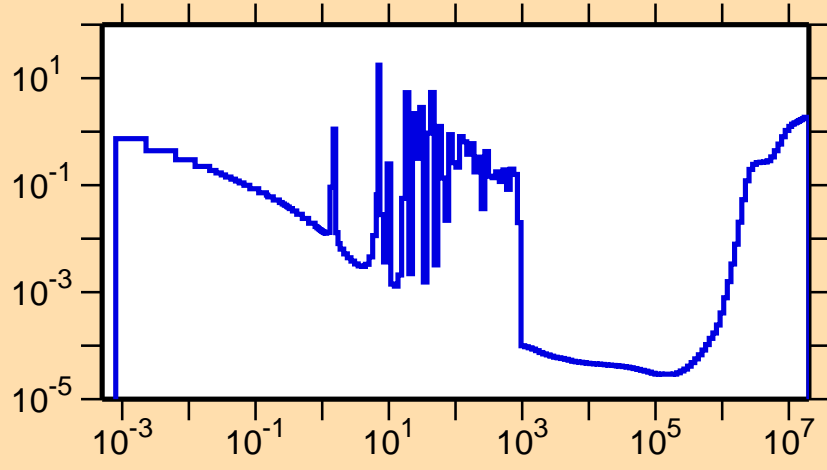
\sigma vs. E for ^{244}\text{Cf}(n,f)
