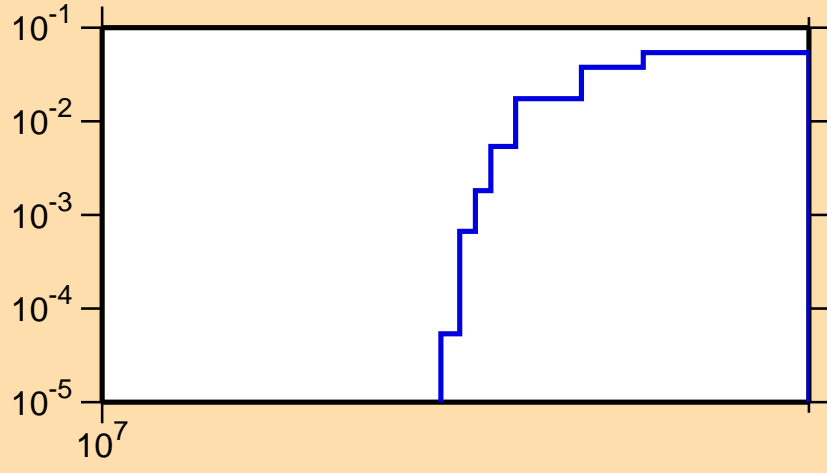
\sigma vs. E for ^{244}\text{Cf}(n,3n)
