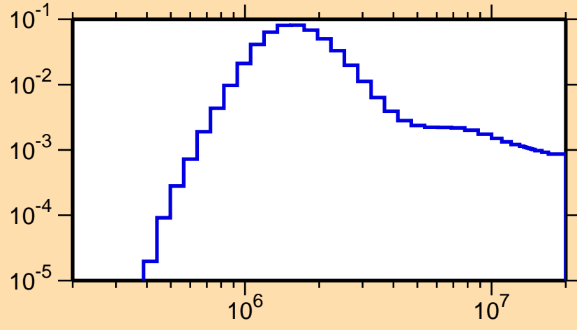
\sigma vs. E for ^{244}\text{Cf}(n,n_4)
