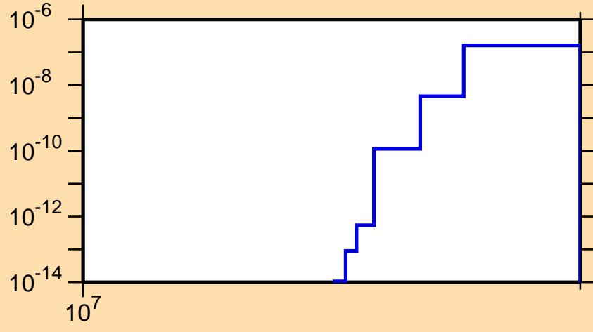
\sigma vs. E for ^{244}\text{Cf}(n,2np)
