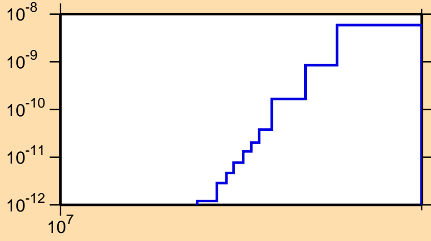
\sigma vs. E for ^{244}\text{Cf}(n,\text{He3})
