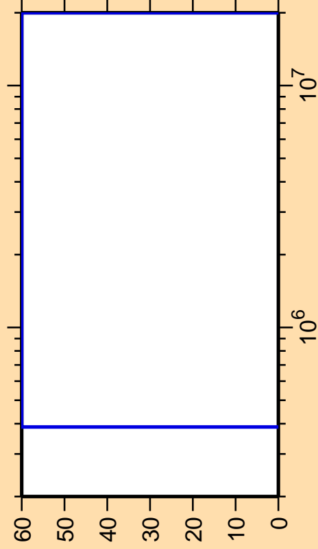
\Delta\sigma/\sigma vs. E for ^{244}\text{Cf}(n,n_4)
