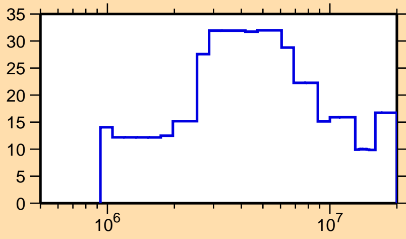
\Delta\sigma/\sigma vs. E for ^{244}\text{Cf}(n,el.)
