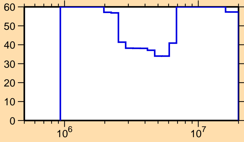
\Delta\sigma/\sigma vs. E for ^{244}\text{Cf}(n,n\text{cont.})
