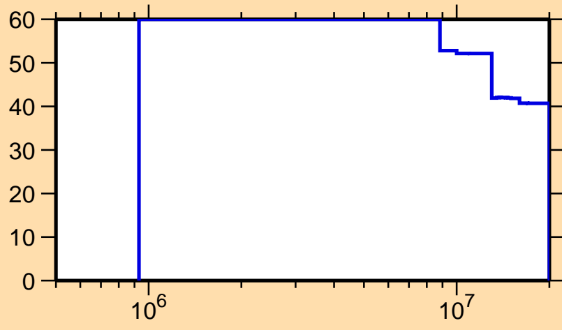
\Delta\sigma/\sigma vs. E for ^{244}\text{Cf}(n,f)
