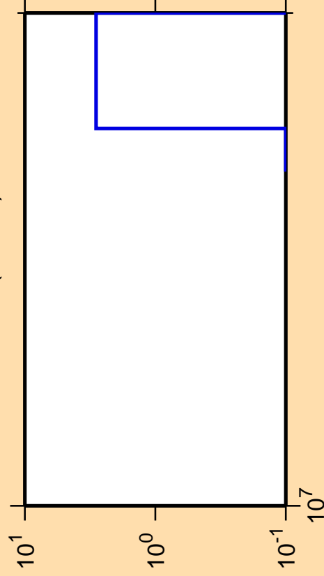
\Delta\sigma/\sigma vs. E for ^{245}\text{Cf}(\text{mt } 34)
