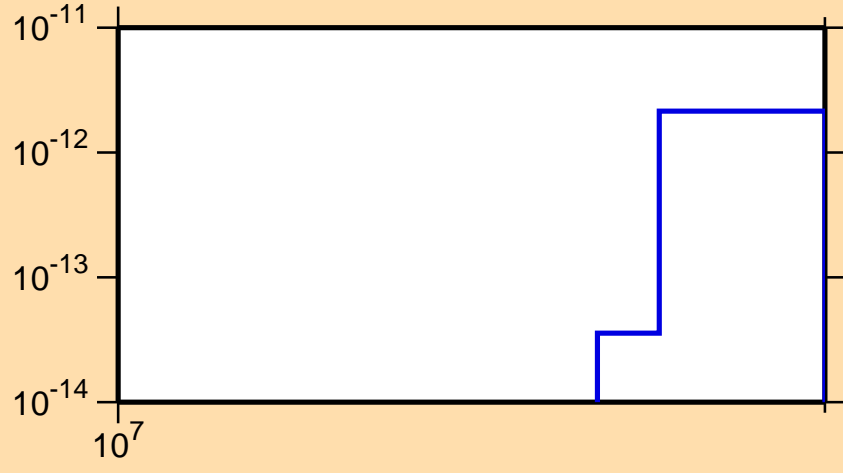
\sigma vs. E for ^{245}\text{Cf}(\text{mt } 34)
