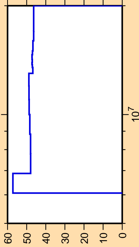
\Delta\sigma/\sigma vs. E for ^{245}\text{Cf}(n,n_1)
