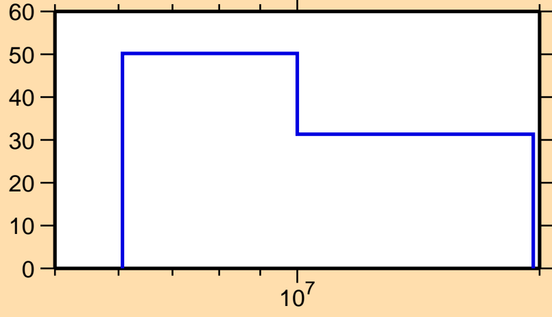
\Delta\sigma/\sigma vs. E for ^{245}\text{Cf}(n,2n)
