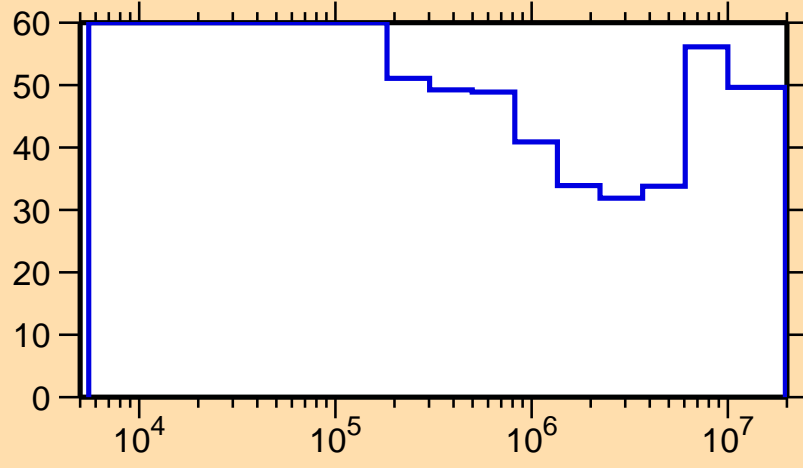
\Delta\sigma/\sigma vs. E for ^{245}\text{Cf}(n,\text{inel.})
