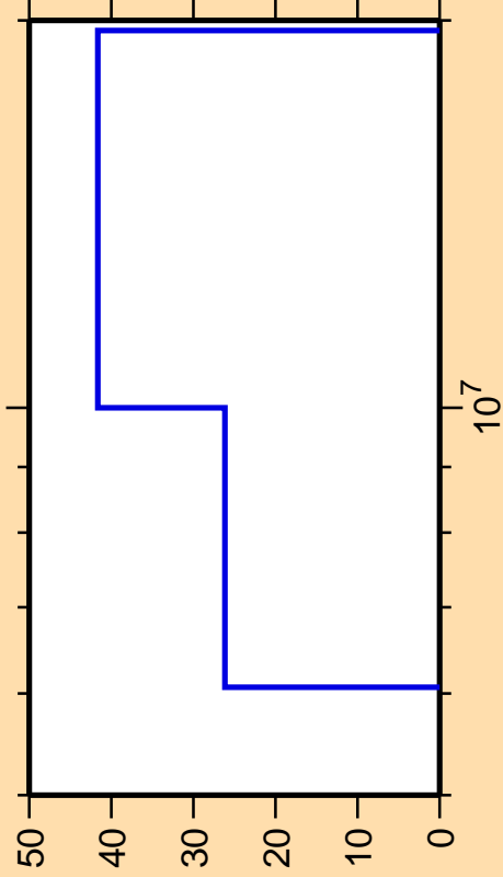
\Delta\sigma/\sigma vs. E for ^{245}\text{Cf}(n,t)
