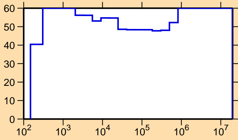
\Delta\sigma/\sigma vs. E for ^{245}\text{Cf}(n,\gamma)
