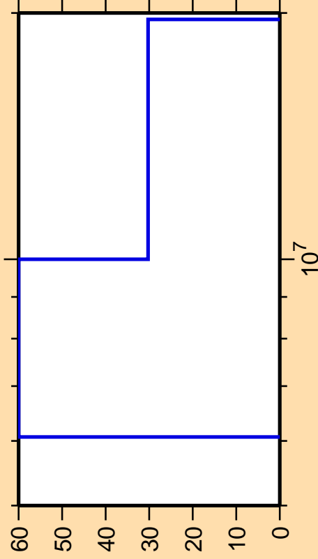
\Delta\sigma/\sigma vs. E for ^{245}\text{Cf}(n,f)
