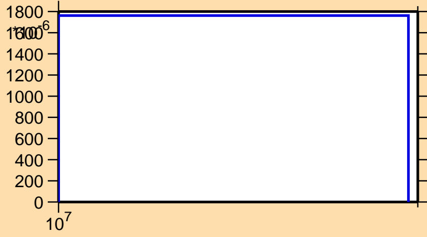
\sigma vs. E for ^{245}\text{Cf}(n,3n\alpha)
