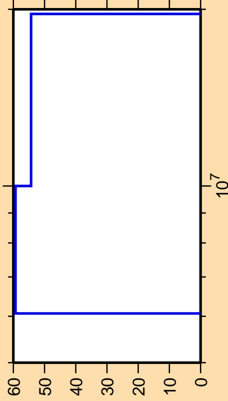
\Delta\sigma/\sigma vs. E for ^{245}\text{Cf}(n,n\text{cont.})
