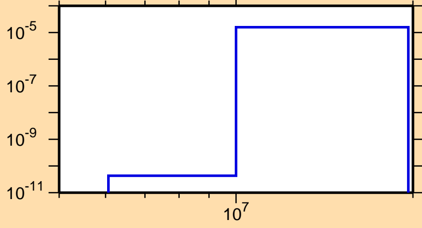
\sigma vs. E for ^{245}\text{Cf}(\text{mt117})
