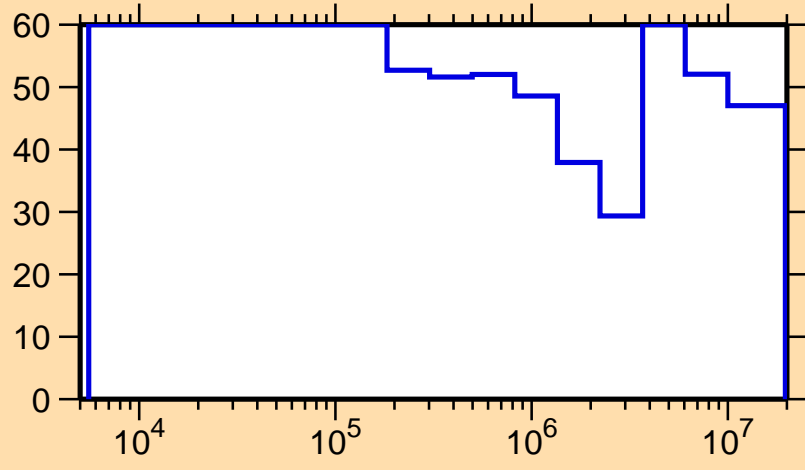
\Delta\sigma/\sigma vs. E for ^{245}\text{Cf}(n,n_1)
