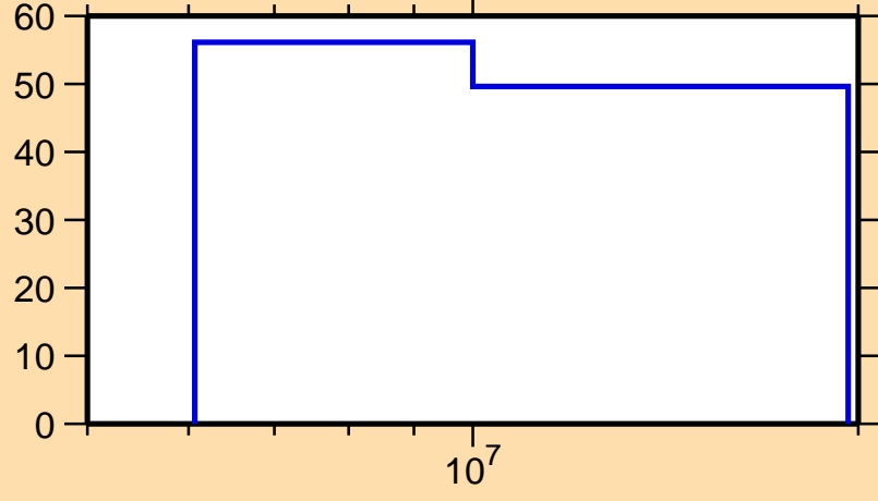
\Delta\sigma/\sigma vs. E for ^{245}\text{Cf}(n,\text{inel.})
