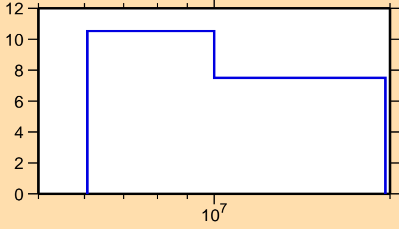
\Delta\sigma/\sigma vs. E for ^{245}\text{Cf}(n,\text{nonel.})
