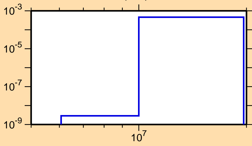
\sigma vs. E for ^{245}\text{Cf}(n,d)
