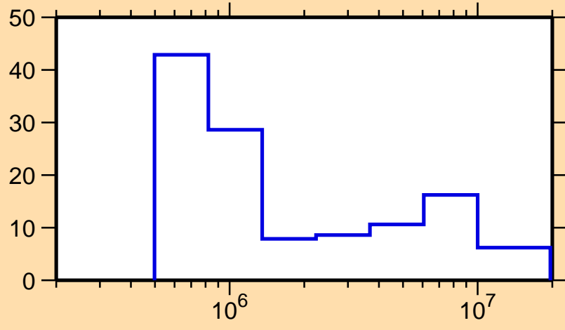
\Delta\sigma/\sigma vs. E for ^{245}\text{Cf}(n,\text{el.})
