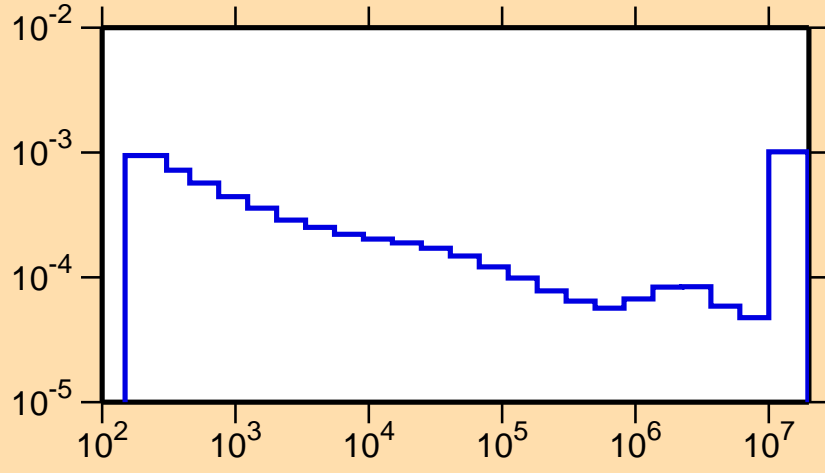
\sigma vs. E for ^{245}\text{Cf}(n,\alpha)
