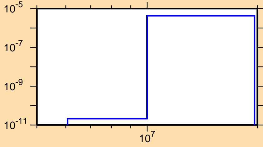
\sigma vs. E for ^{245}\text{Cf}(\text{mt } 45)
