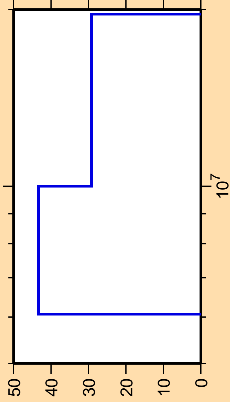
\Delta\sigma/\sigma vs. E for ^{245}\text{Cf}(n,d)
