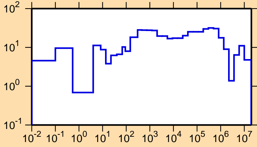
\Delta\sigma/\sigma vs. E for ^{245}\text{Cf}(n,\text{tot.})
