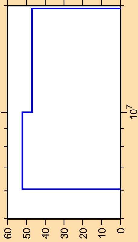
\Delta\sigma/\sigma vs. E for ^{245}\text{Cf}(n,n_1)
