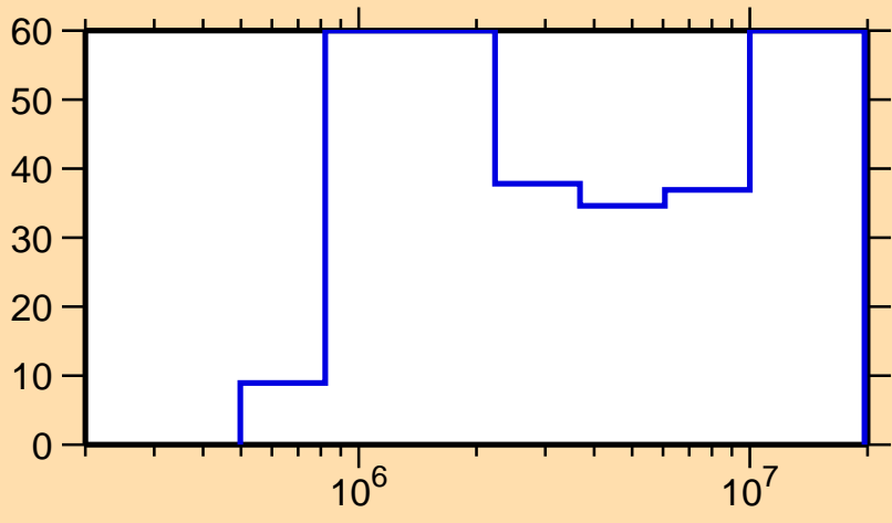
\Delta\sigma/\sigma vs. E for ^{245}\text{Cf}(n,p)
