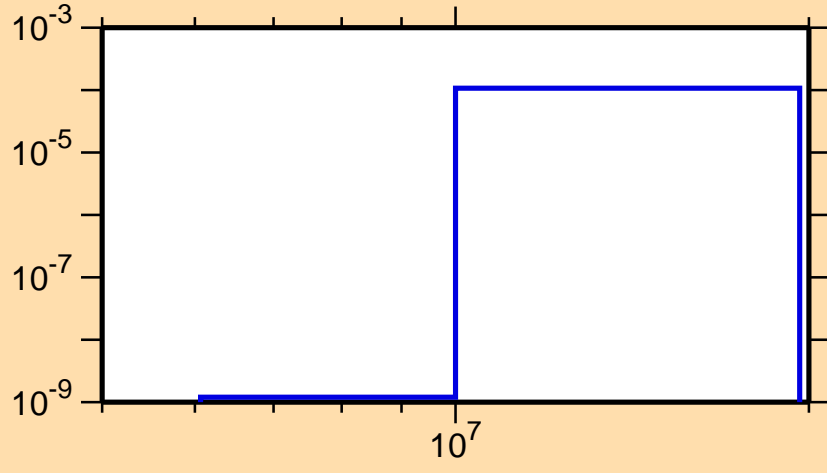
\sigma vs. E for ^{245}\text{Cf}(n,np)
