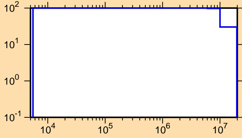
\Delta\sigma/\sigma vs. E for ^{245}\text{Cf}(n,f)
