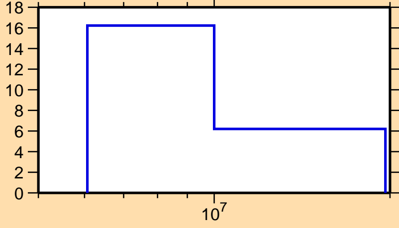
\Delta\sigma/\sigma vs. E for ^{245}\text{Cf}(n,\text{el.})
