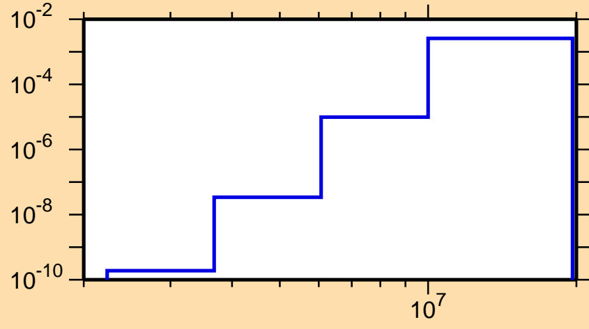
\sigma vs. E for ^{245}\text{Cf}(n,p\alpha)
