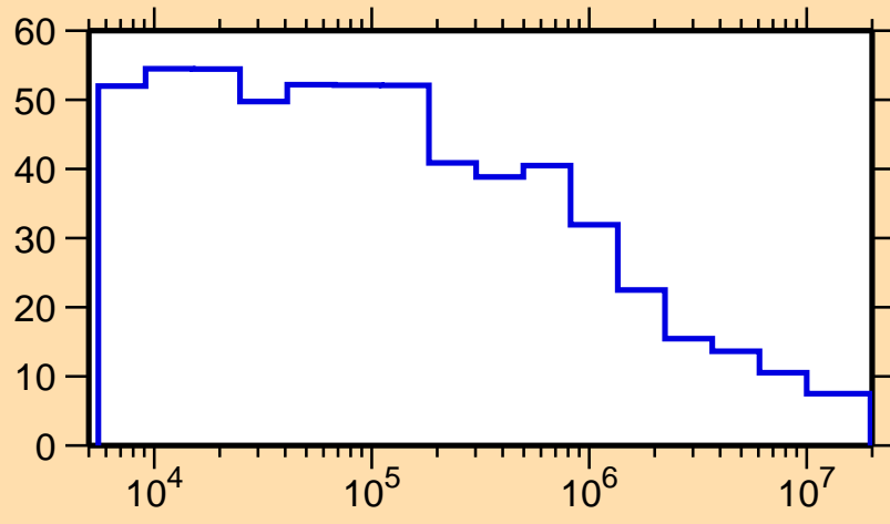
\Delta\sigma/\sigma vs. E for ^{245}\text{Cf}(n,\text{nonel.})
