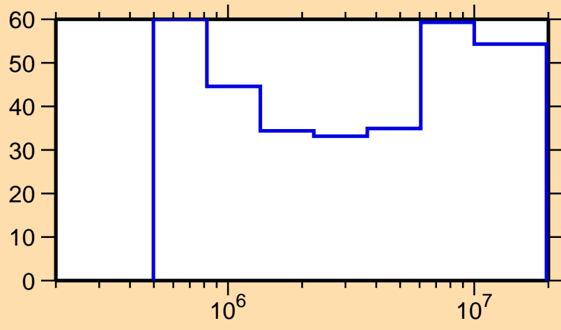
\Delta\sigma/\sigma vs. E for ^{245}\text{Cf}(n,n\text{cont.})
