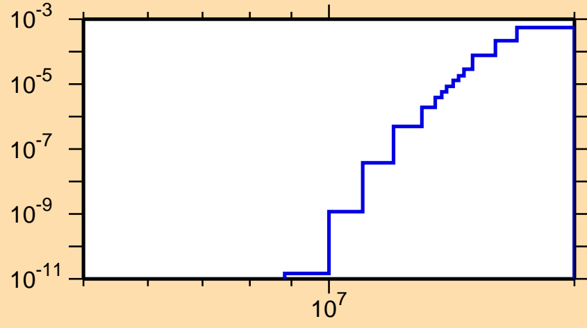
\sigma vs. E for ^{246}\text{Cf}(\text{mt117})
