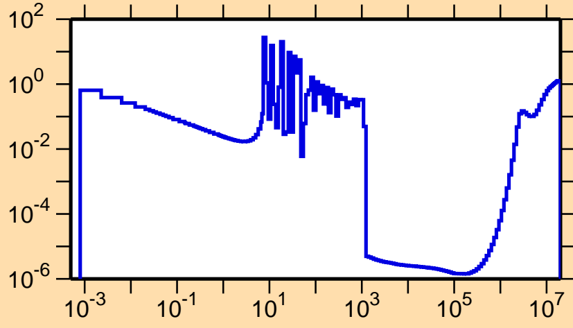
\sigma vs. E for ^{246}\text{Cf}(n,f)
